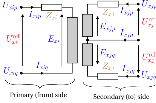
Figure 6: Center tap transformer equivalent circuit
