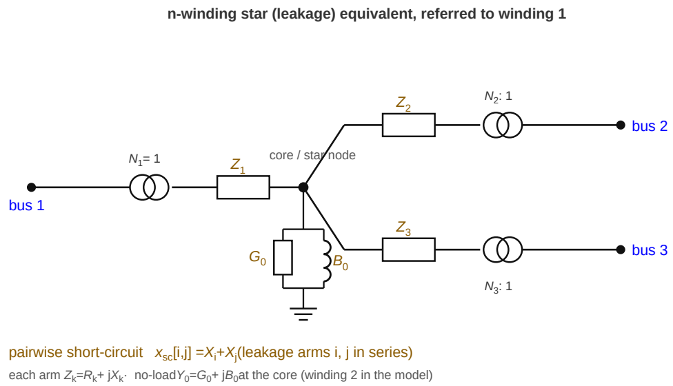
Figure 17.8: n-winding star (leakage) equivalent, referred to winding 1: each winding contributes a leakage arm to a common core node, the no-load shunt sits at the core, and each winding pair (i,j) has its own short-circuit reactance x_{sc}[i,j] = X_i + X_j .
