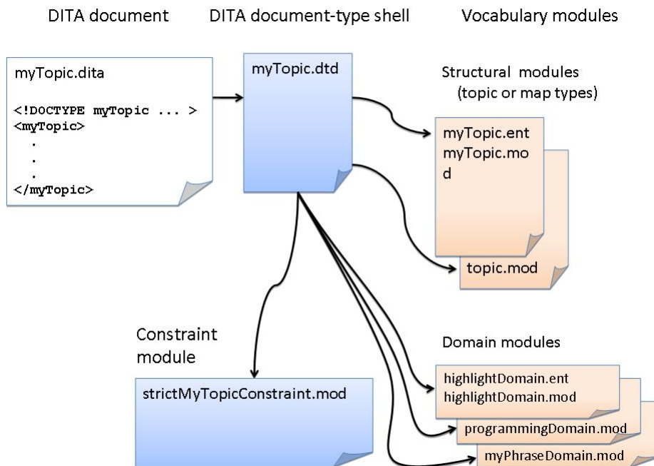
Figure 3: Instances, modules, and declarations
