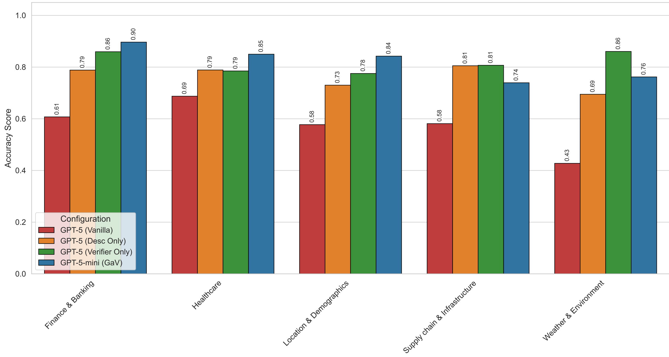
Ablation Study: Impact of Architecture Components (GPT-5-mini (GaV))
