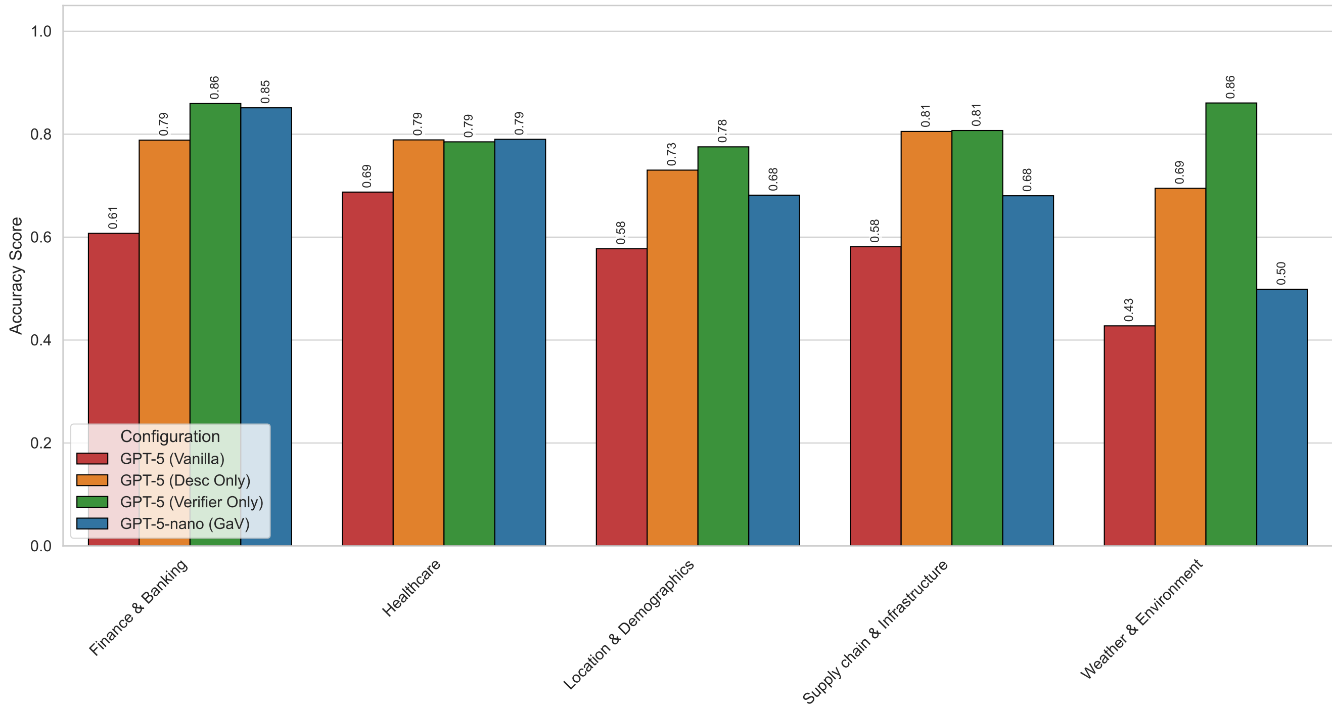
Ablation Study: Impact of Architecture Components (GPT-5-nano (GaV))
