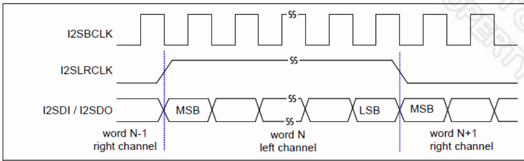
Fig2. MSB Justified Timing Diagram (PCM=0, Format=1)
