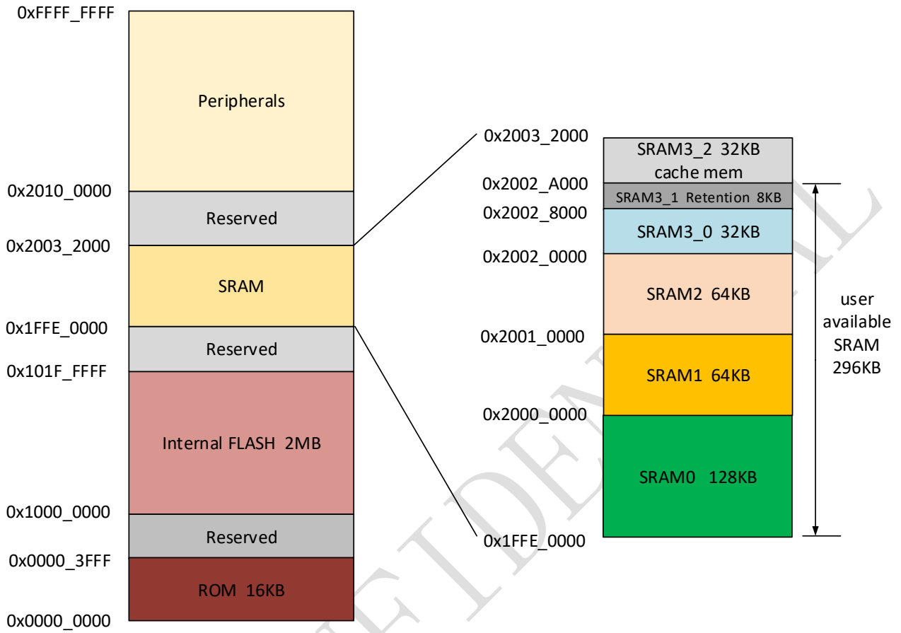
Figure 1-2 LN8825B Memory Map
