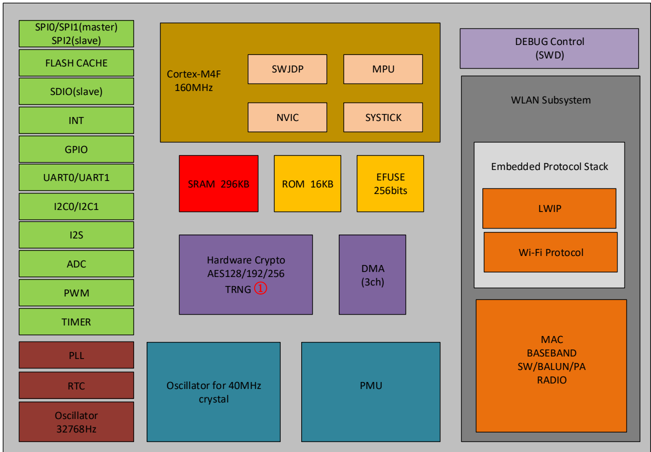
Figure 1-1 LN8825X block diagram
