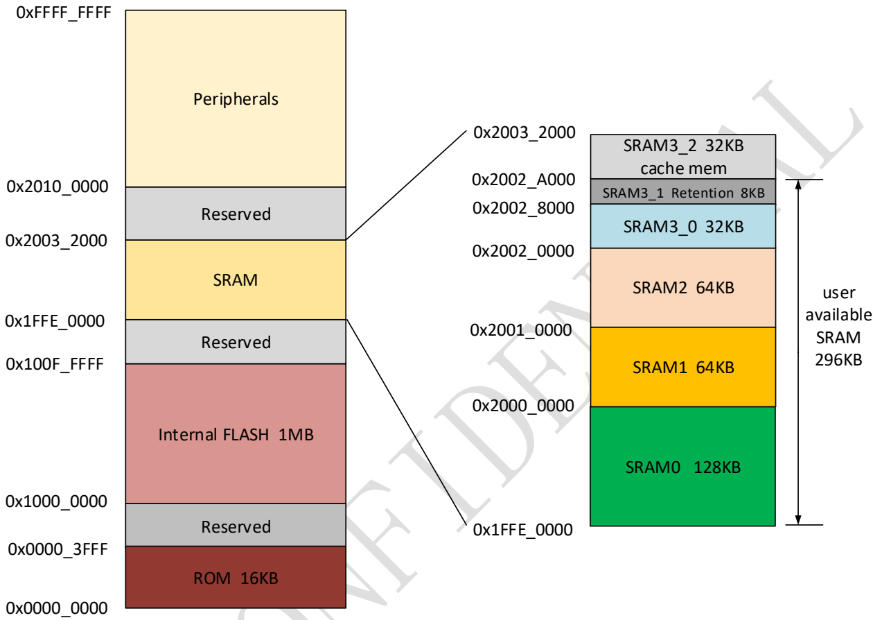
Figure 1-2 LN8825A Memory Map
