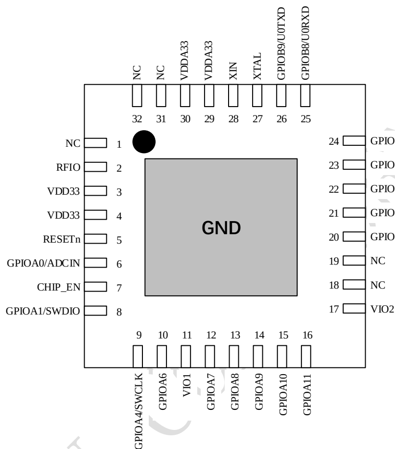
Figure 4-1 LN8825X Pin Layout
