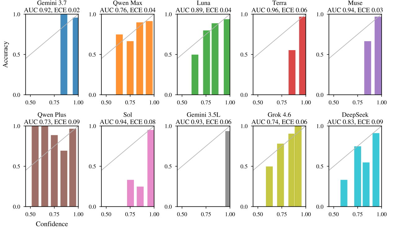
Figure 7: Reliability diagrams for the ten field configurations (bars: accuracy within confidence bins; line: perfect calibration). Titles give confidence AUC and ECE. Terra discriminates best (AUC 0.963) despite a mid-table EAS; Qwen3.7 Plus and Grok 4.6 are confidently wrong.
