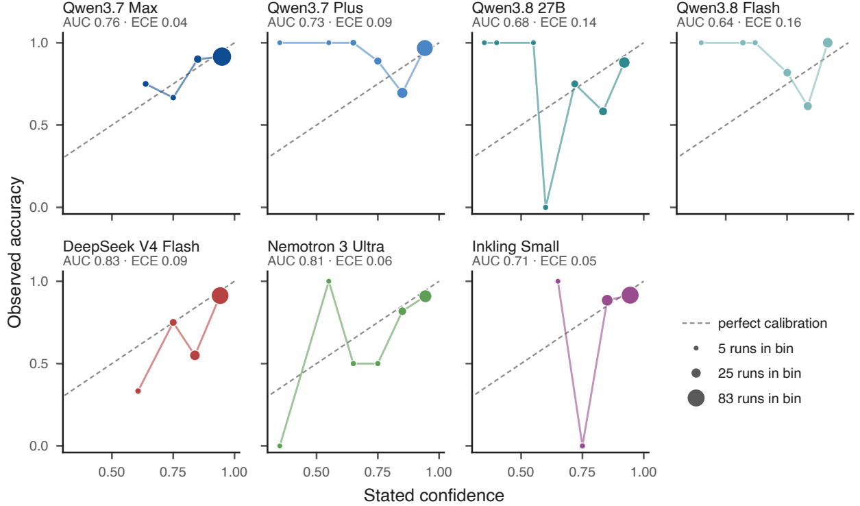
Figure 7: Reliability diagrams for the 7 field-eligible configurations (points: accuracy within each confidence bin, sized by the number of runs in it; dashed line: perfect calibration). Titles give confidence AUC and ECE. DeepSeek V4 Flash discriminates best (AUC 0.826) despite a low-to-mid EAS; Qwen3.8 Flash and Qwen3.8 27B are confidently wrong.
