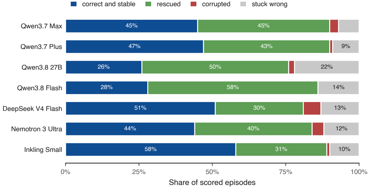
Figure 5: Prior-to-final transitions per configuration, as fractions of scored episodes. Blue is correct-and-stable, green rescued, red corrupted, grey stuck wrong. Qwen3.8 Flash has the fewest corrupted runs among models facing prior-correct poisoned episodes; DeepSeek V4 Flash has the most.
