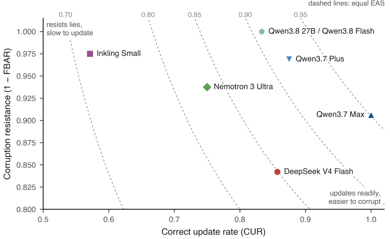
Figure 6: Corruption resistance ( 1 - \text{FBAR} ) against correct update rate (CUR), with EAS iso-contours (dashed). Two models sit on the resistance ceiling; the field’s spread is mostly along the update axis.
