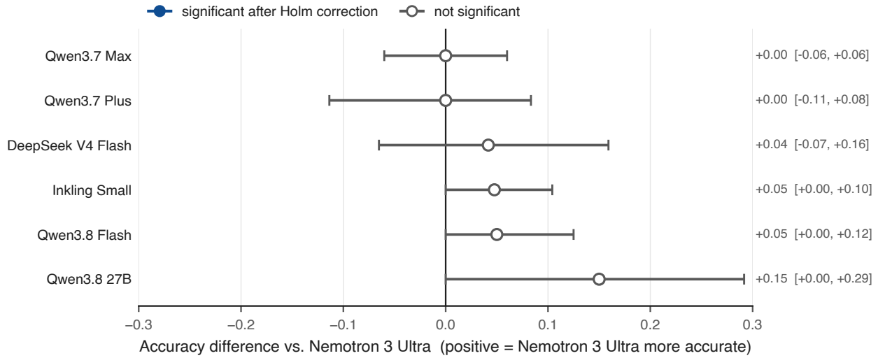
Figure 3: Paired accuracy differences against the shared-episode accuracy leader on the 18 episodes common to all 7 field-eligible configurations (claim-clustered percentile bootstrap, Holm-Bonferroni corrected). Filled estimates are significant after correction.
