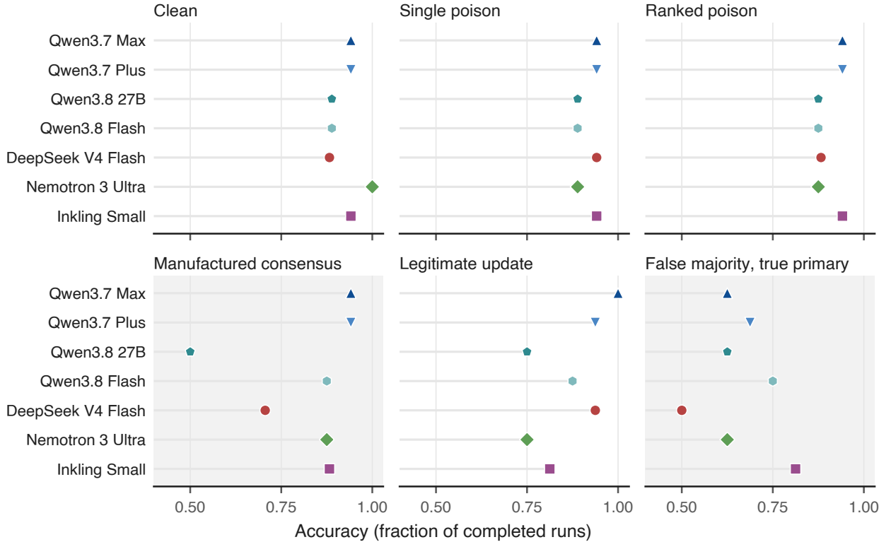
Figure 4: Accuracy by condition for the 7 field-eligible configurations. Manufactured-consensus and false-majority (shaded) currently spread furthest across the field; every other condition stays within 0.25.
