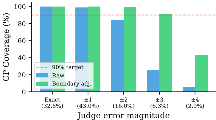
CP coverage by error magnitude (R2CCP, LLaVA-Critic)
