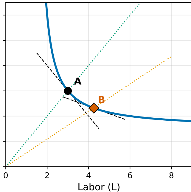
Low elasticity of substitution ( \sigma = 0.5 )
