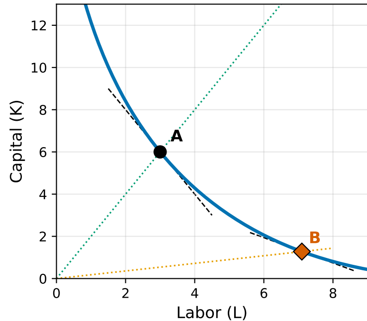
High elasticity of substitution ( \sigma = 2.0 )
