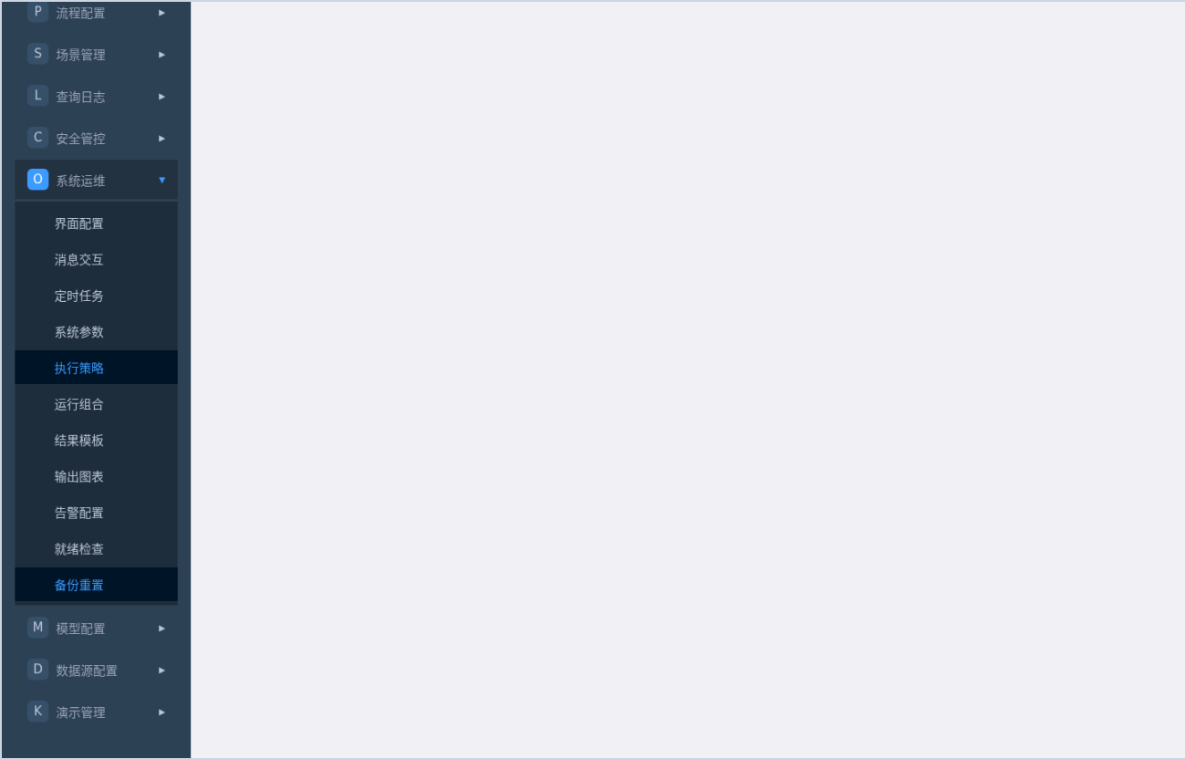
图4-7 备份与重置
