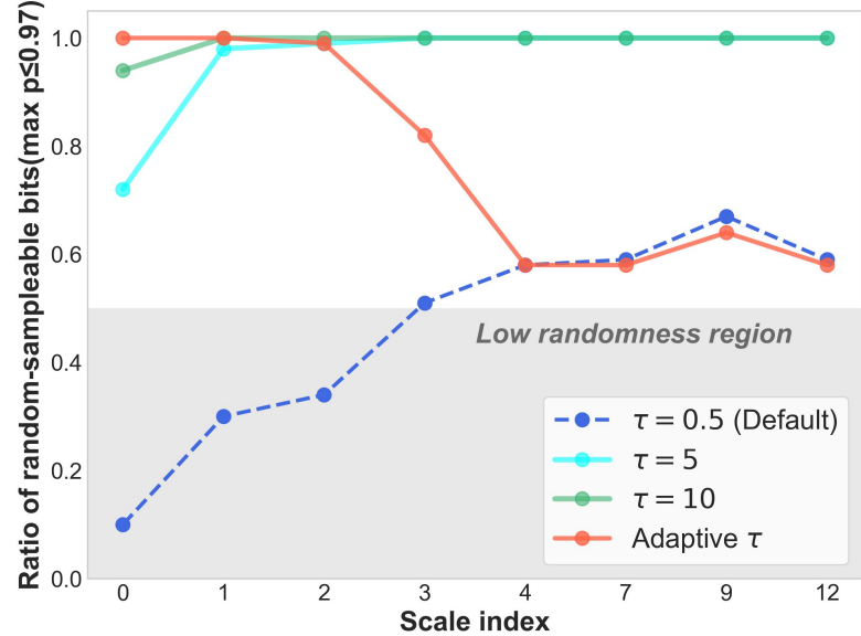
(b) The proportion of bits exhibiting randomness across different scale
