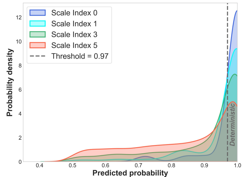
(a) Probability density of output probabilities at different scales
