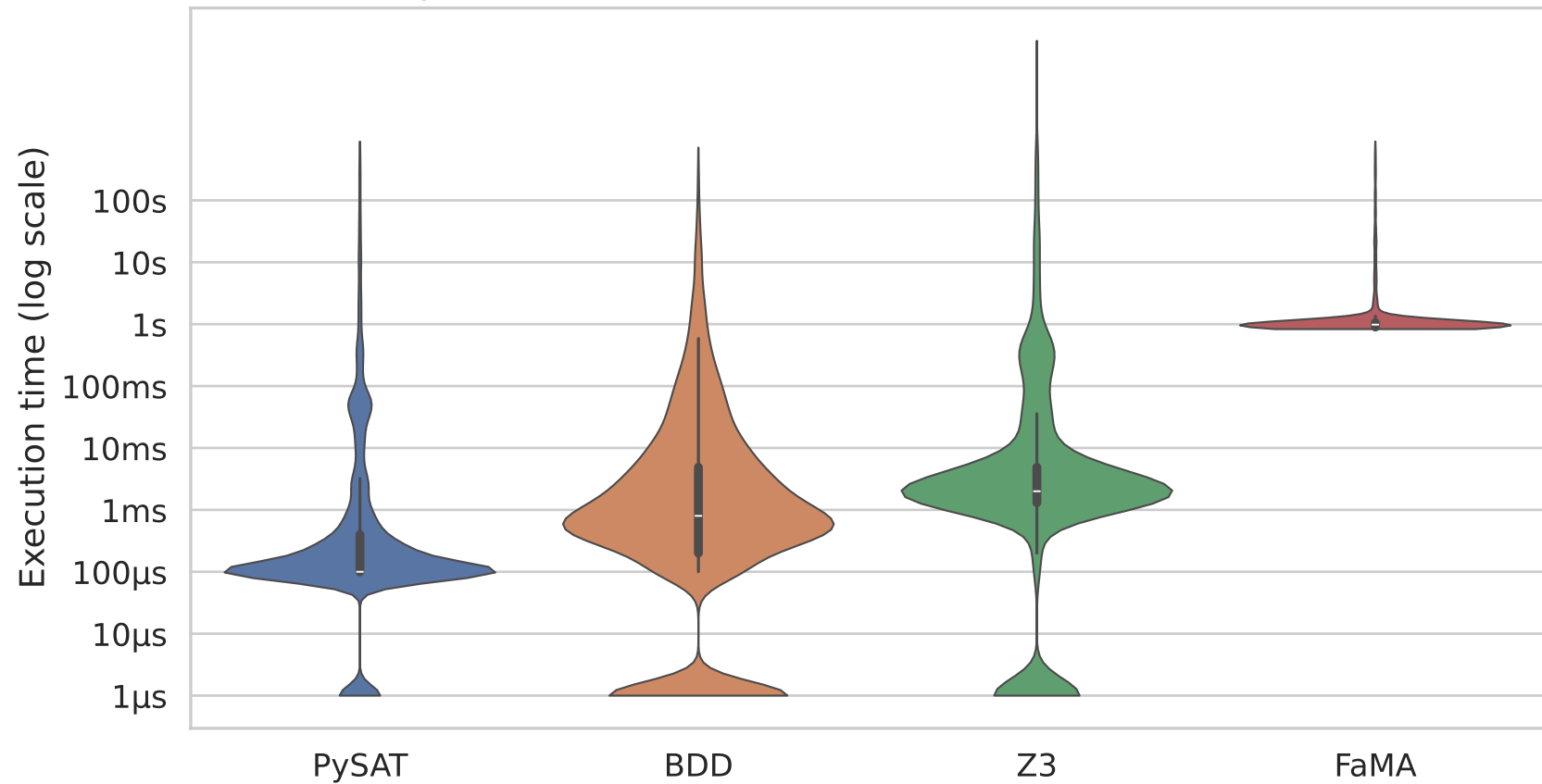
Figure 2 — Execution Time Distribution (successful runs)
