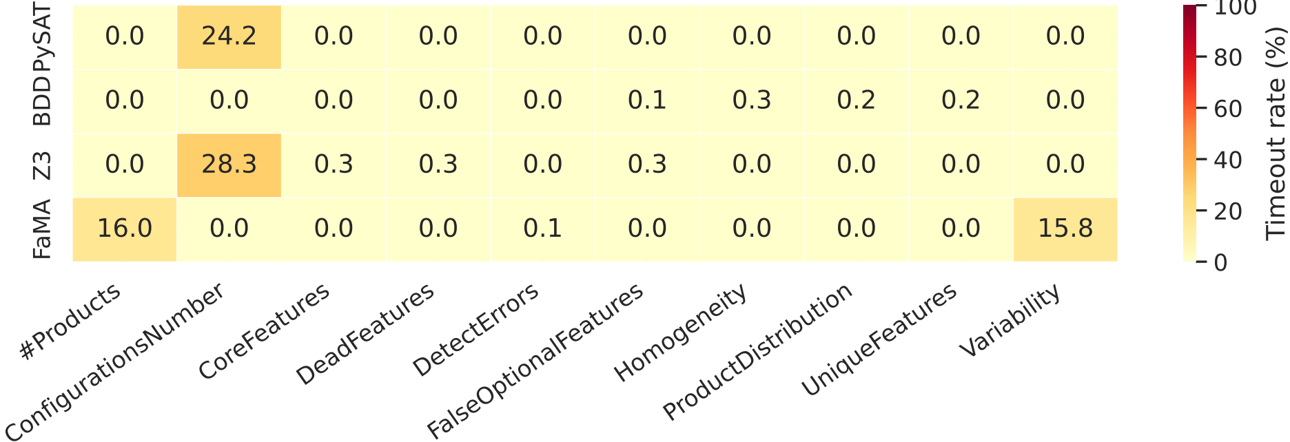
Figure 3 — Timeout Rate by Solver × Operation (%)
