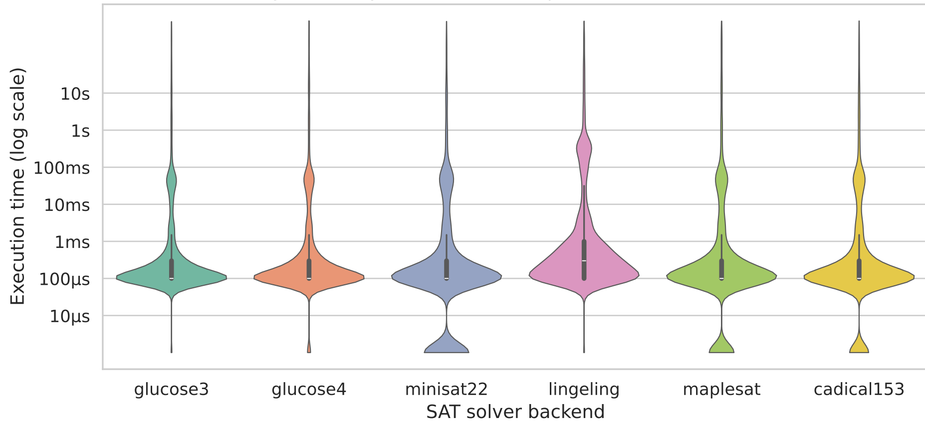
Figure 6 — PySAT Backend Comparison (successful runs)
