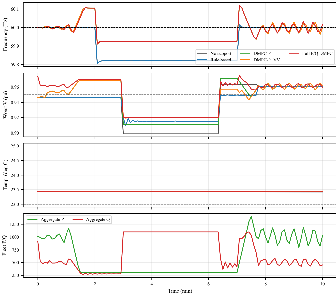
Upstream source-sag event
