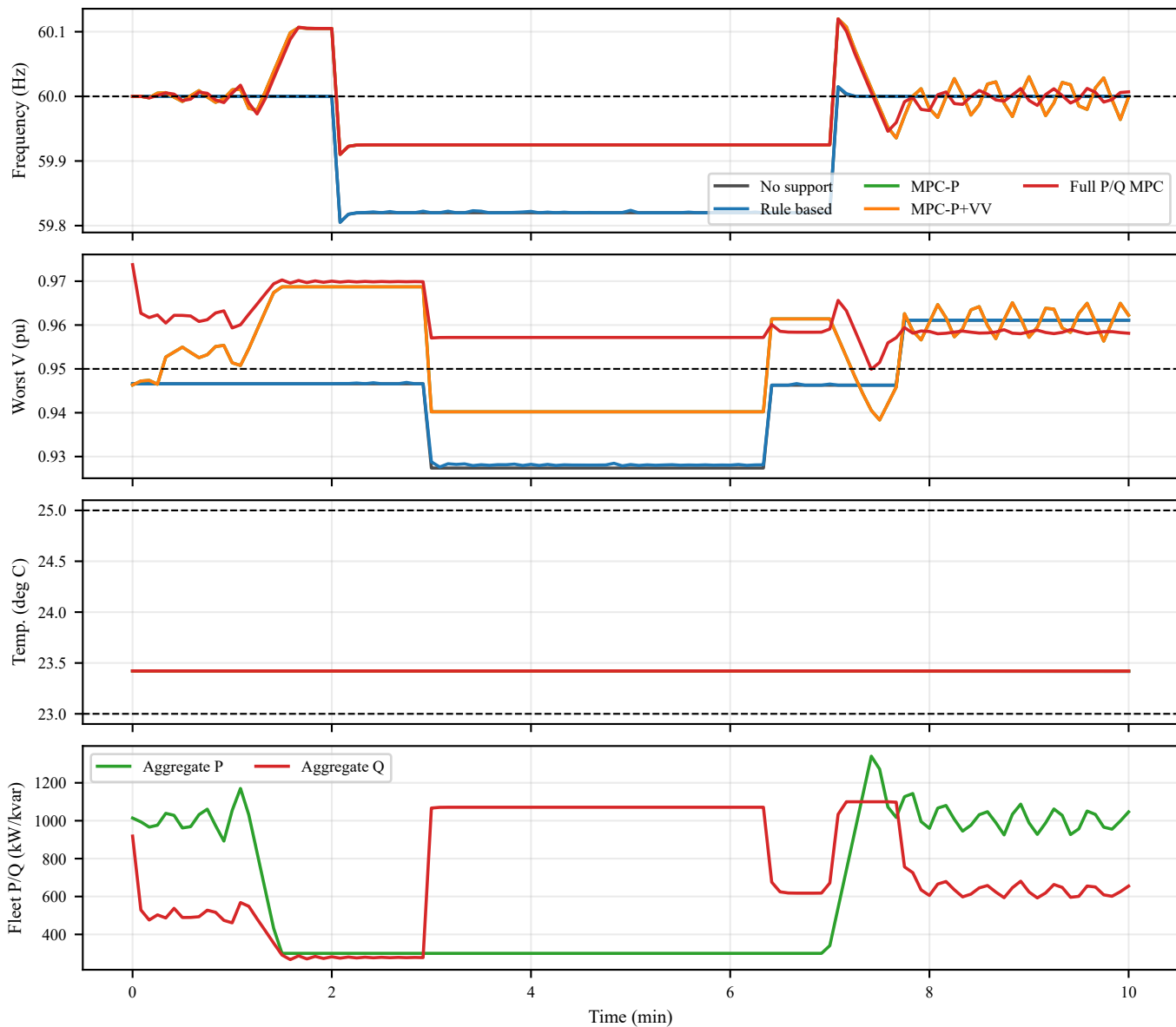
Feeder-local load stress event
