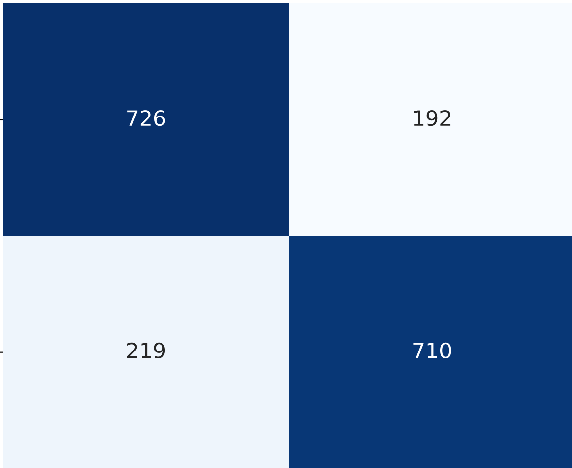
Confusion Matrix (Hold-out Set)
