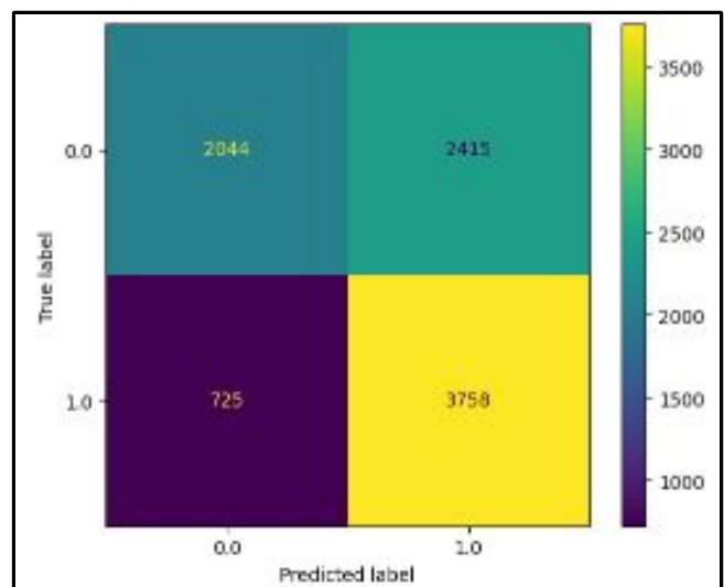
Confusion matrix of logistic regression model
