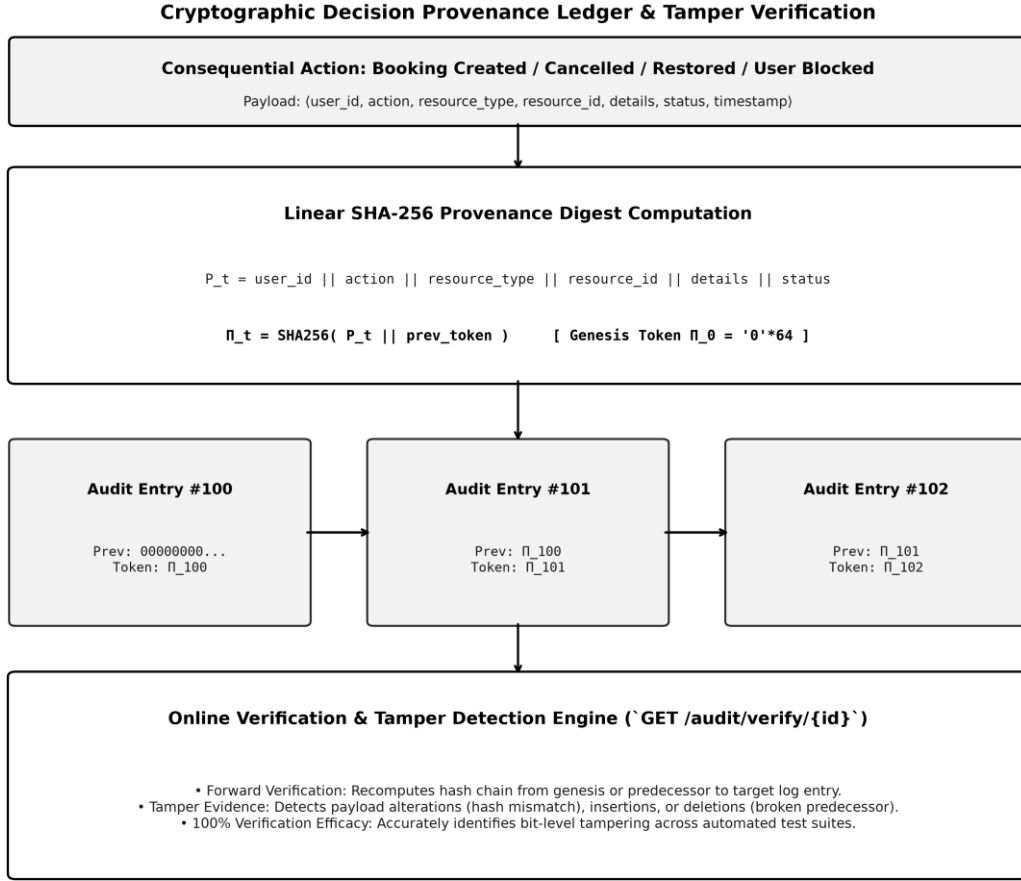
Fig. 6. SHA-256 hash-chained provenance ledger: payload serialization, chained digest computation, and online tamper-detection verification.
