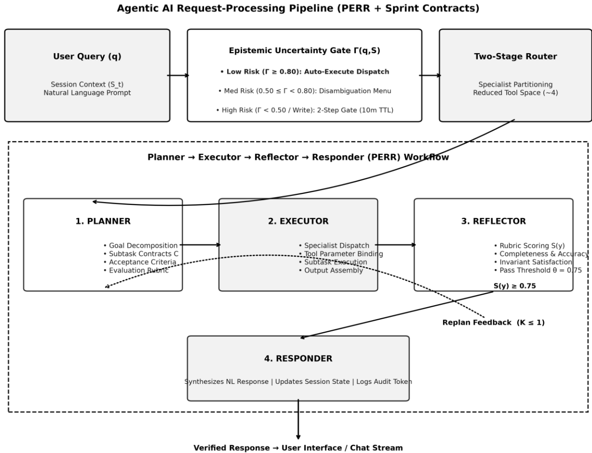
Fig. 2. Agentic request-processing pipeline: uncertainty harness, intent routing, and the PERR (Planner–Executor–Reflector–Responder) execution graph with bounded replanning.
