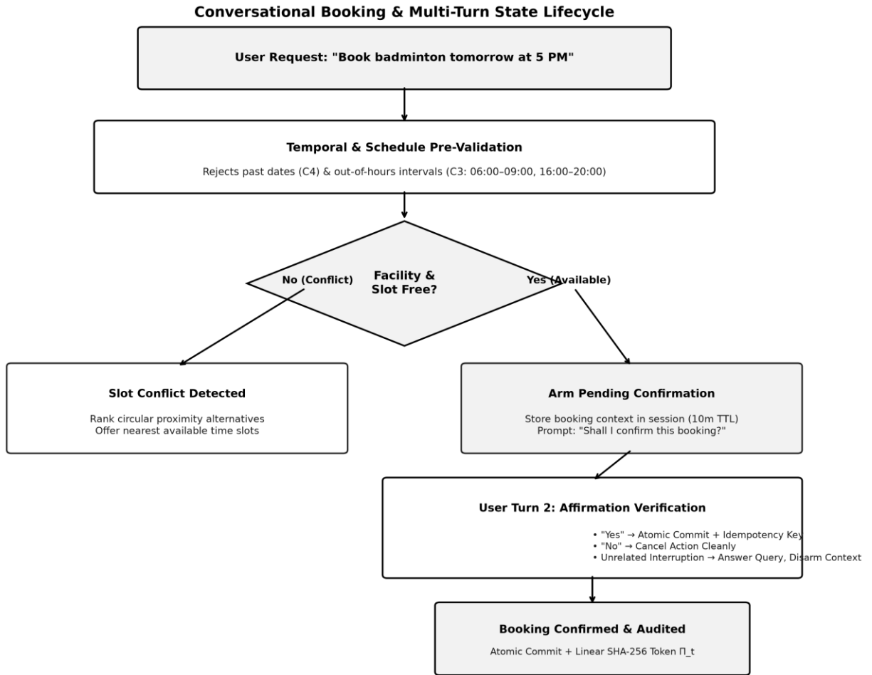
Fig. 4. Conversational booking lifecycle: pre-validation, availability check, two-step confirmation, and provenance logging.
