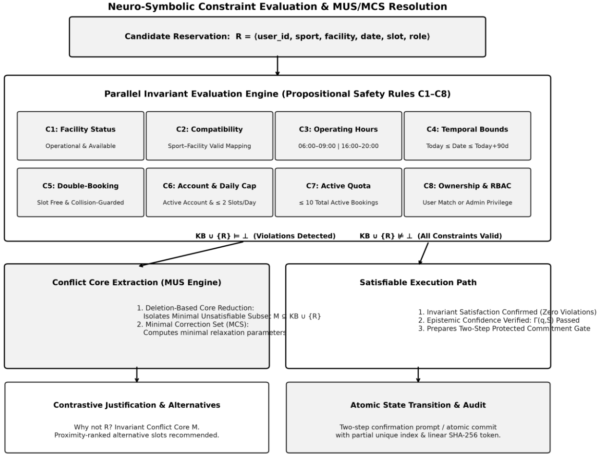
Fig. 3. Parallel invariant evaluation followed by MUS-based conflict-core extraction (unsatisfiable path) or direct commitment (satisfiable path).
