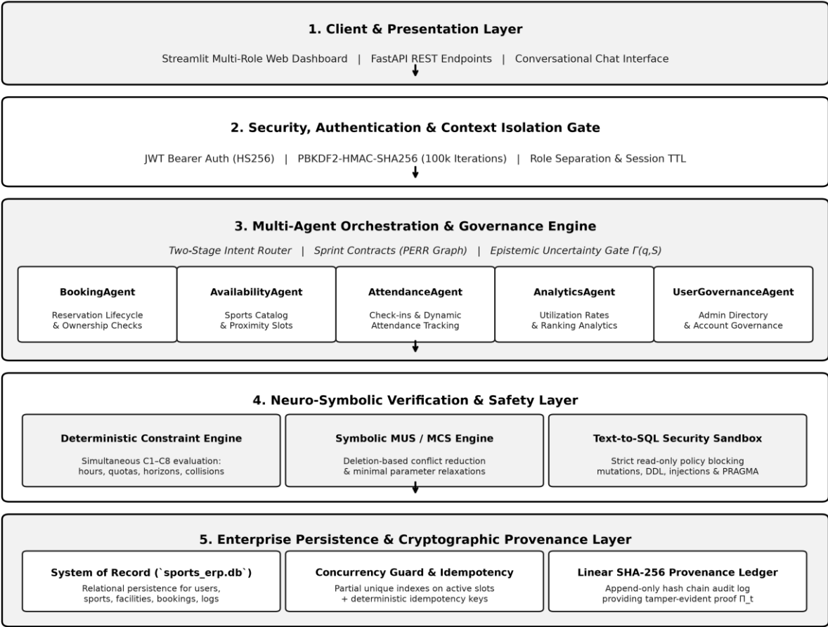
Fig. 1. Five-layer system architecture: client/presentation, security & context isolation, multi-agent orchestration, neuro-symbolic verification, and persistence/provenance.
