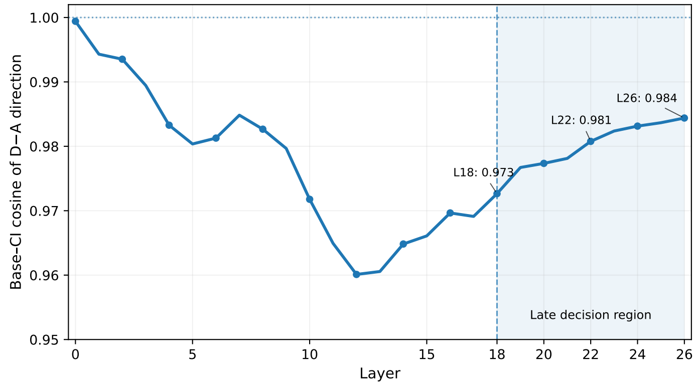
Base and CI preserve a highly aligned privacy contrast
