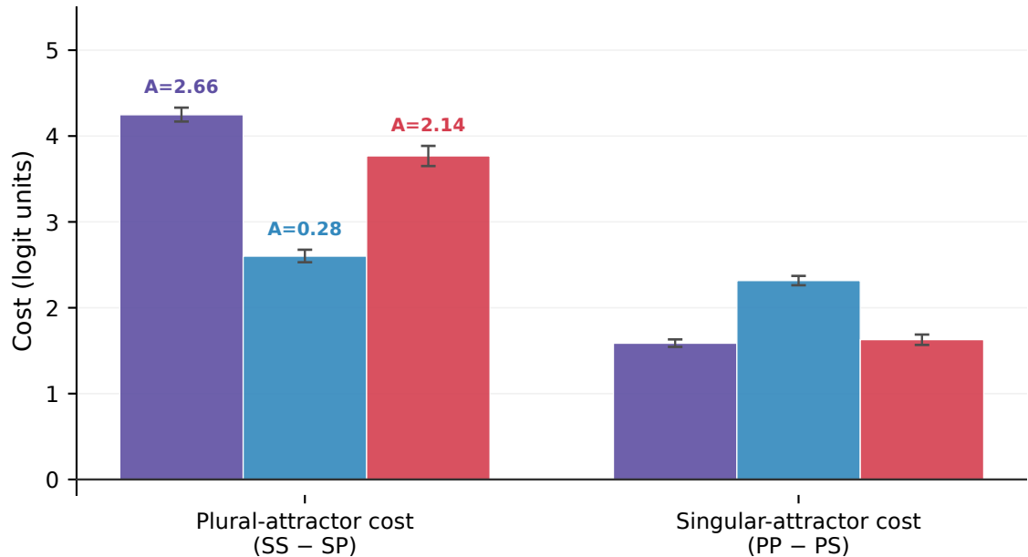
(b) Attractor costs
