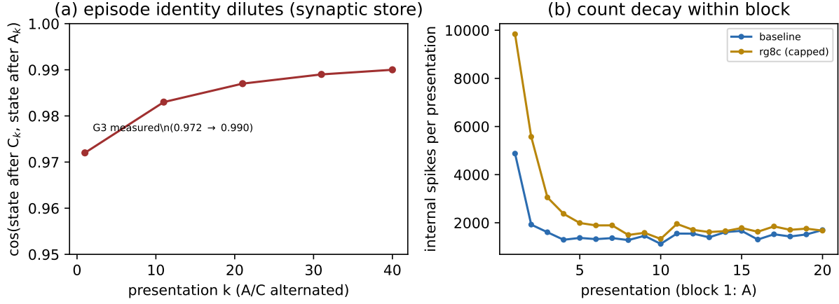
Figure 4: Information dilution across repeated presentations. Left: convergence of the synaptic store after adjacent A and C presentations under alternation (cosine 0.972 \rightarrow 0.990 ; [20]). Right: per-presentation internal spike counts decay within a blocked block (baseline run), the count-level face of the same dilution. Both measured from preserved artifacts.
