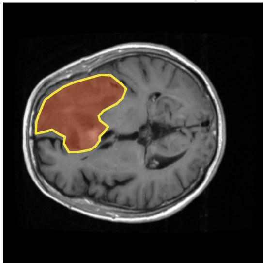
Class Distribution
