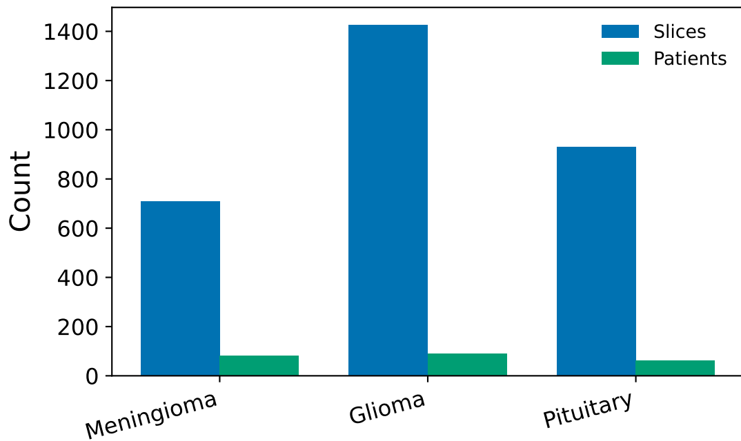
Class Distribution
