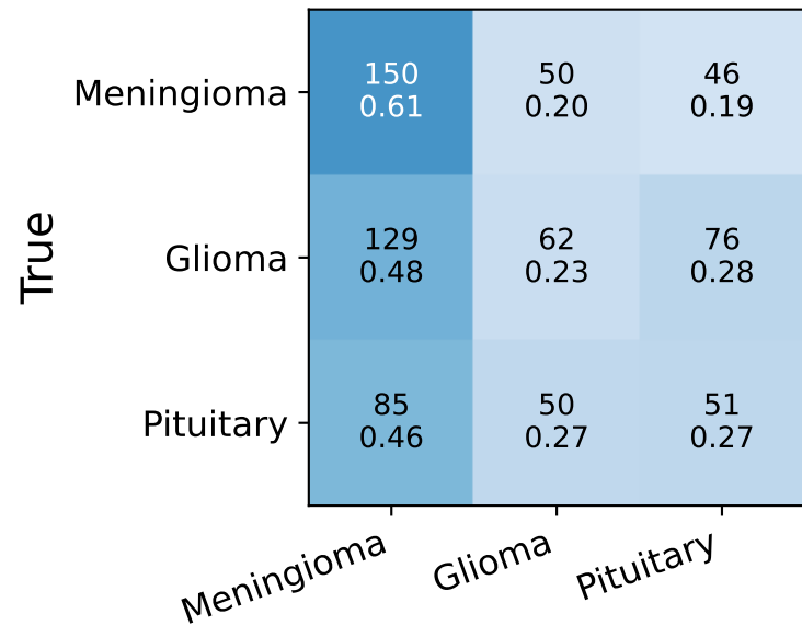
Per-Class Recall
