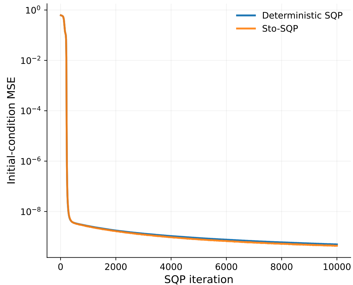
Transport equation: initial-condition MSE
