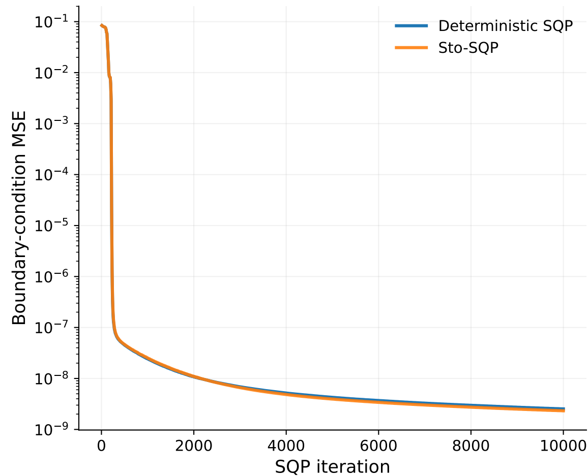
Transport equation: boundary-condition MSE
