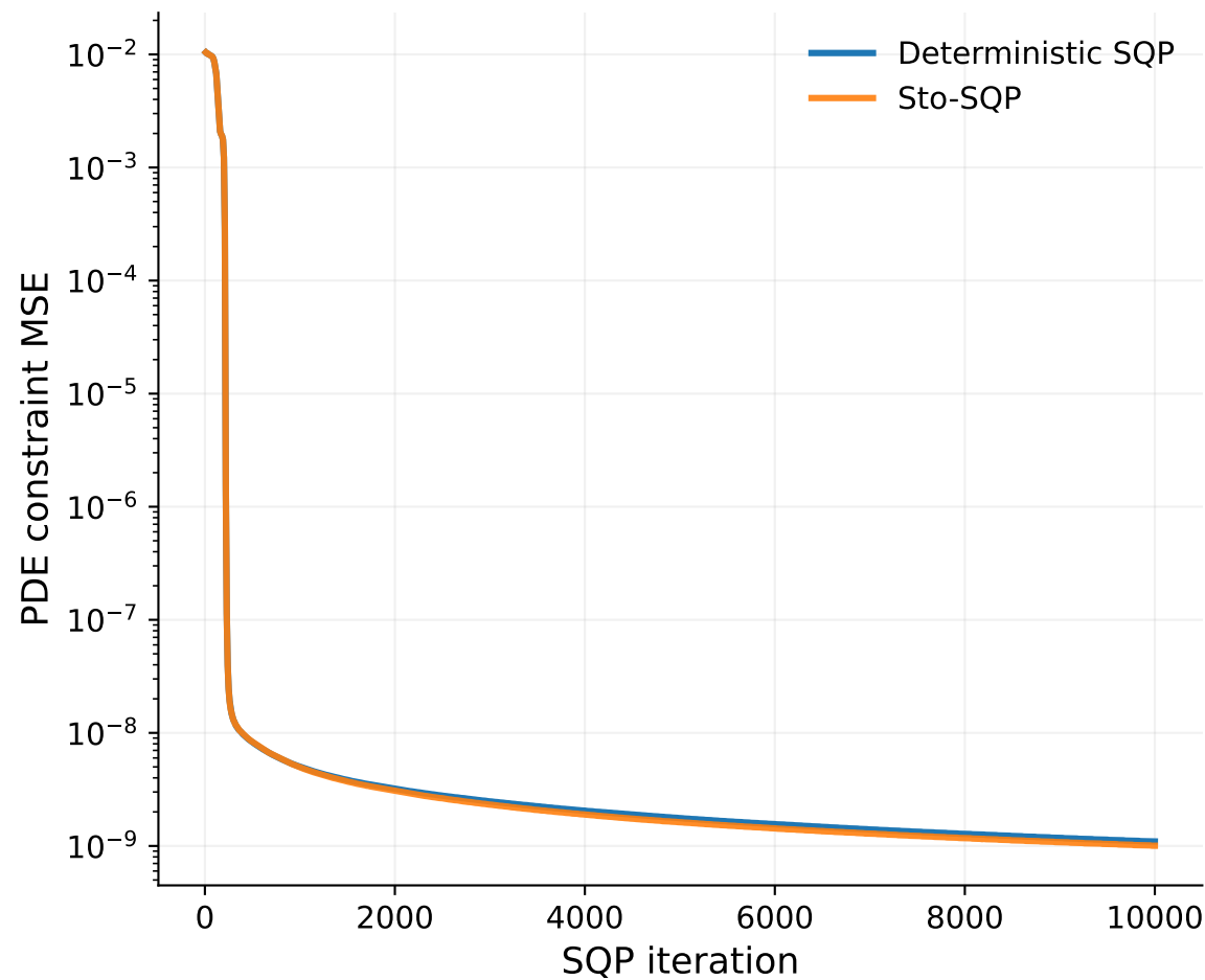
Transport equation: PDE constraint MSE
