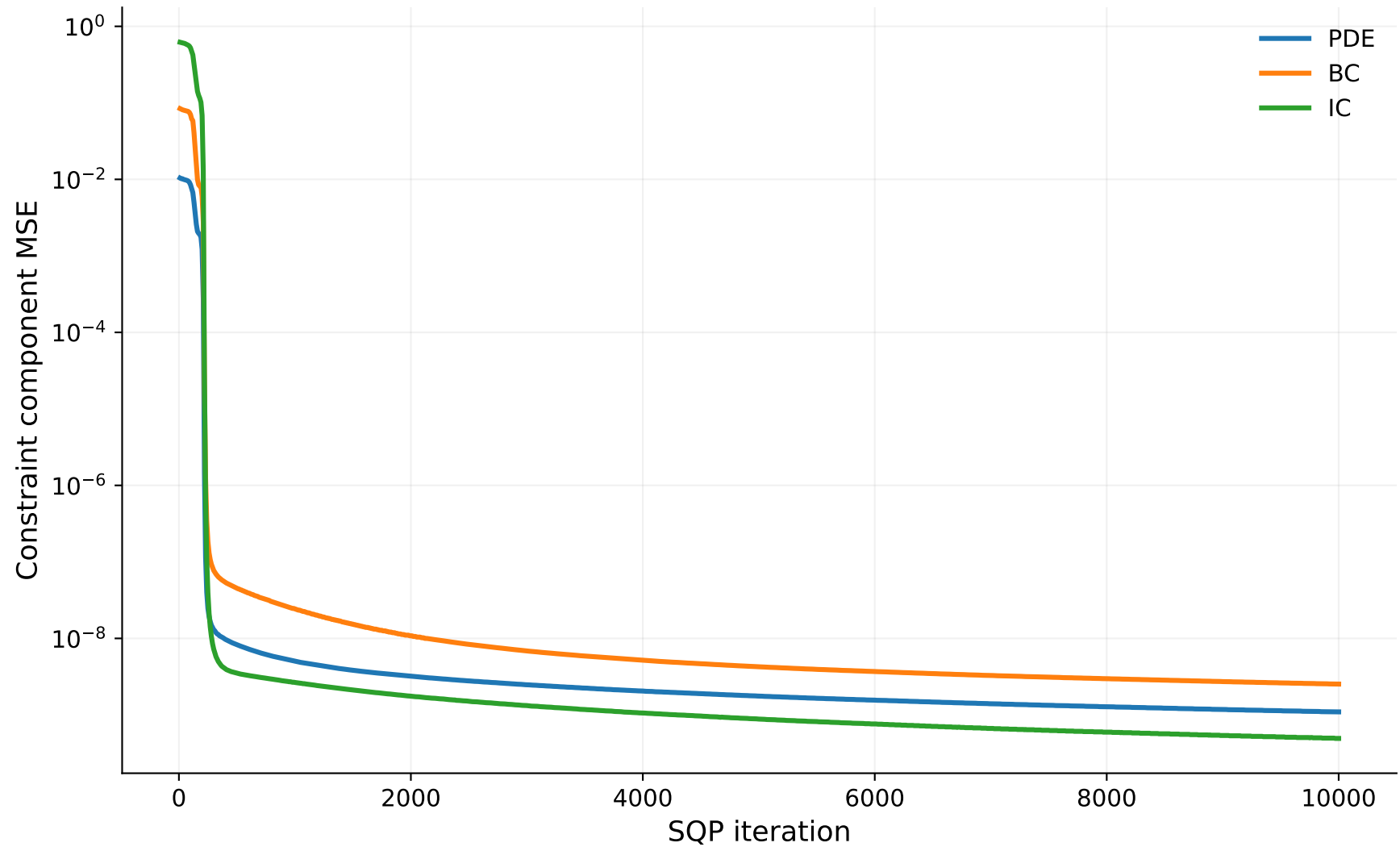
Transport equation: deterministic SQP constraint components
