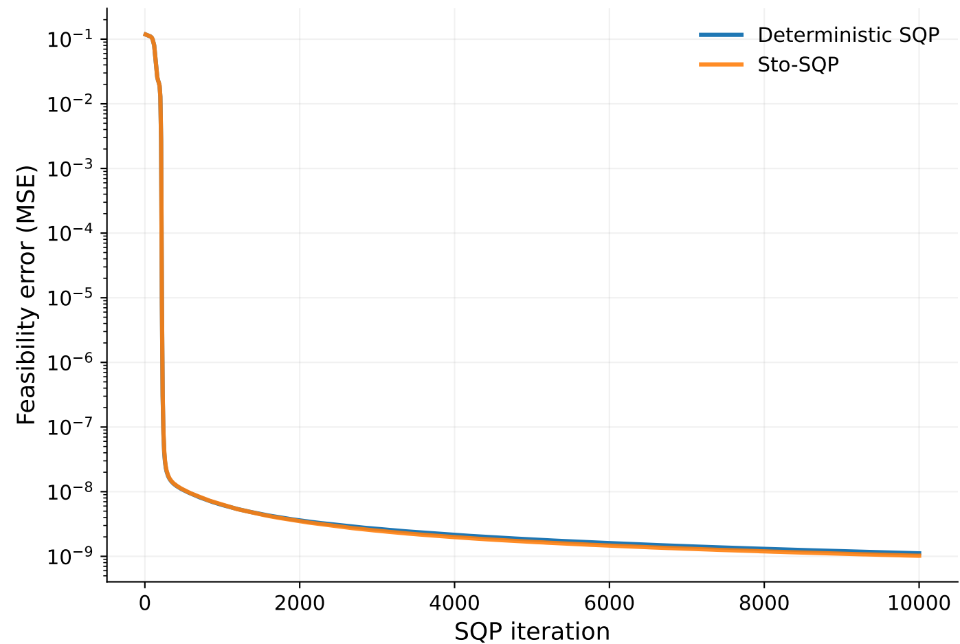
Transport equation: feasibility error
