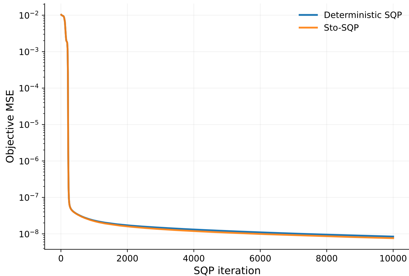
Transport equation: objective MSE
