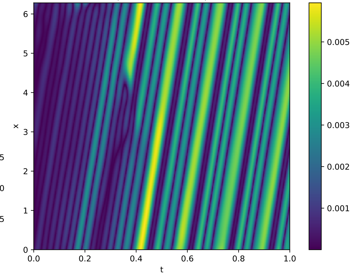
|Prediction - Exact|
