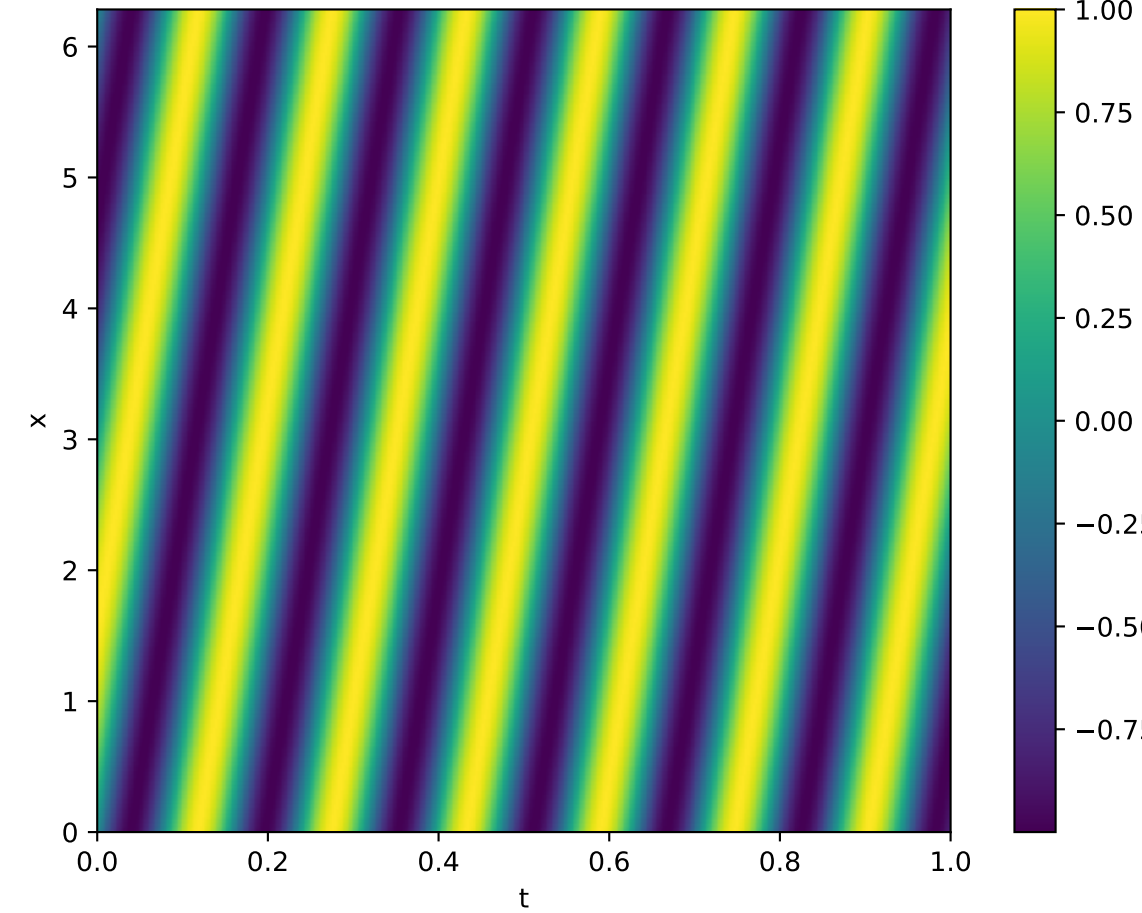
SQP-PINN Prediction
