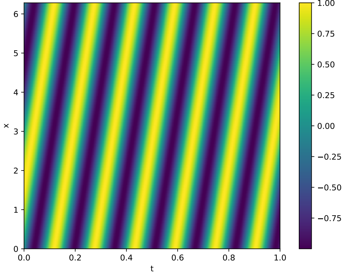
Exact
