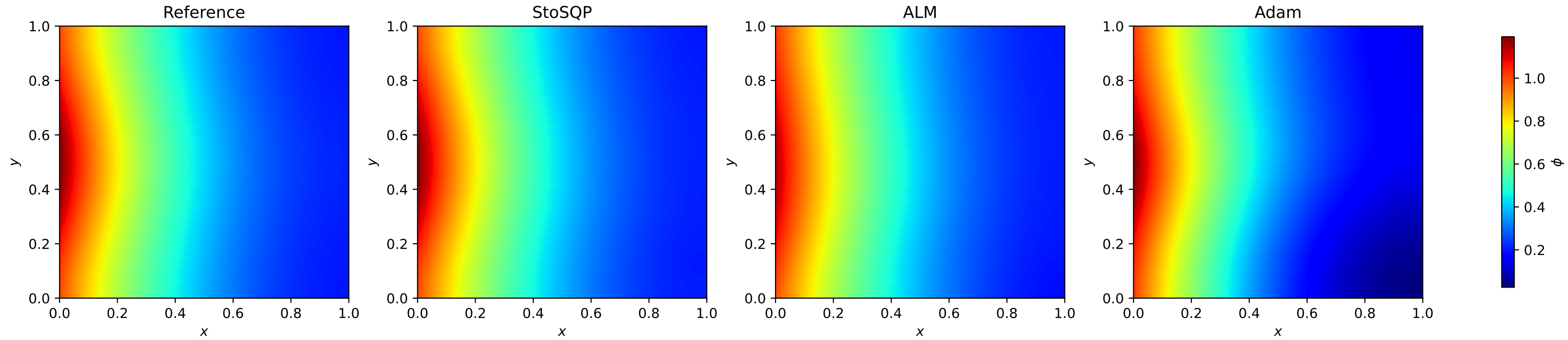
Final-time neutron flux field \phi at t = 1.000
