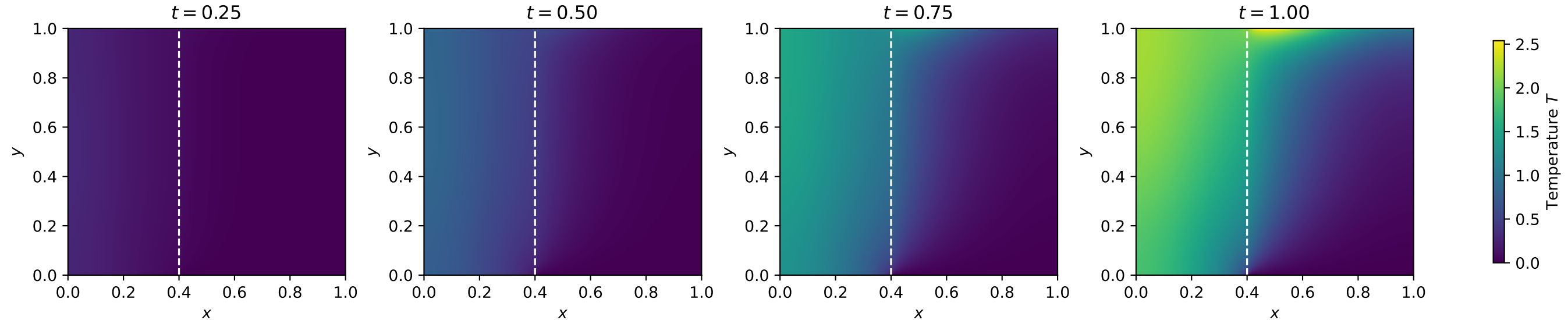
Reference temperature T(x, y, t)
