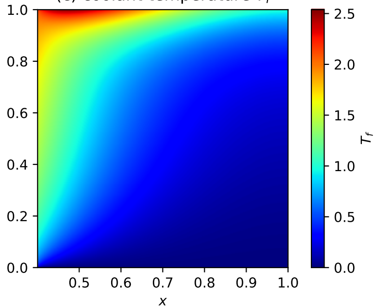
(c) coolant temperature T_f
