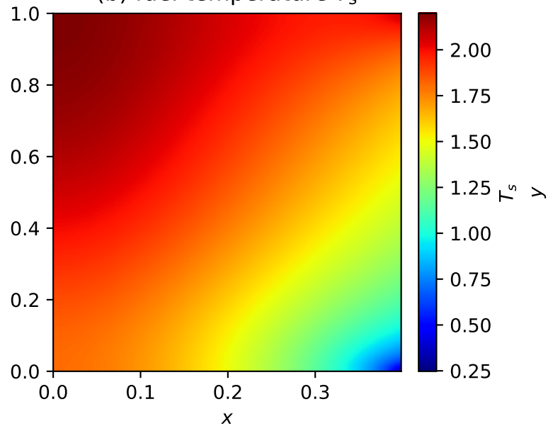
(b) fuel temperature T_s
