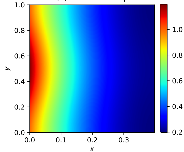
(a) neutron flux \phi
