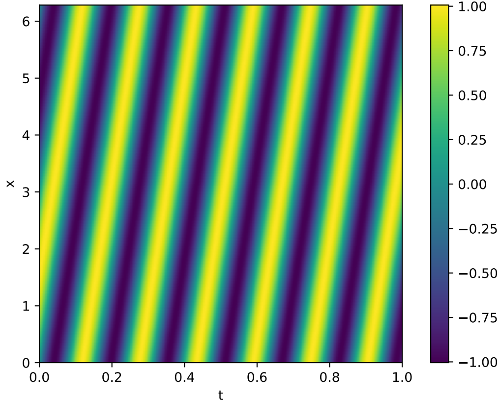
Exact
