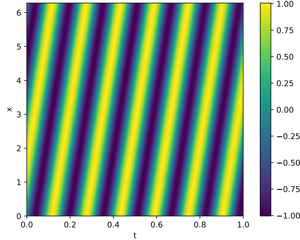
ALM-PINN Prediction
