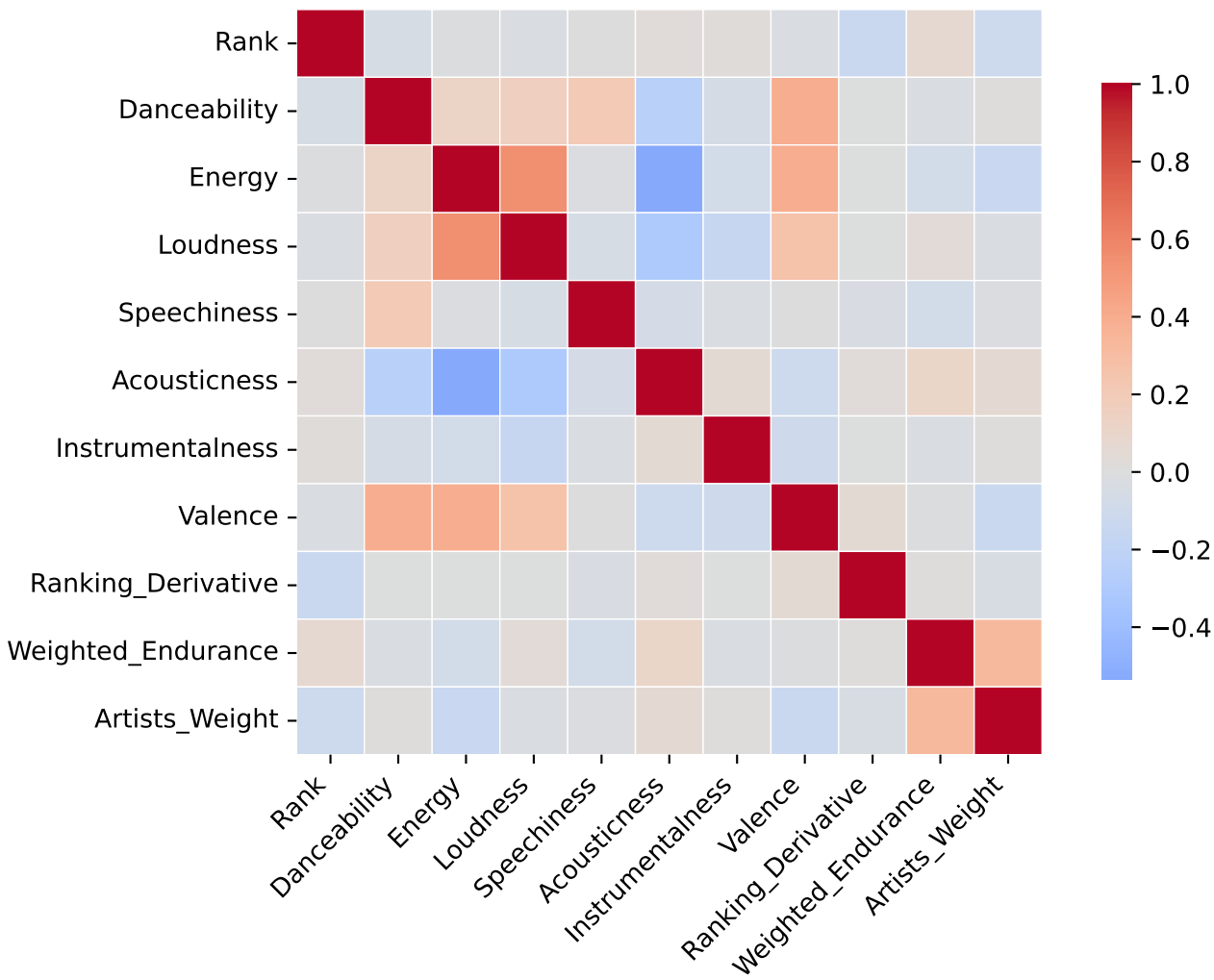
Feature Correlation Matrix
