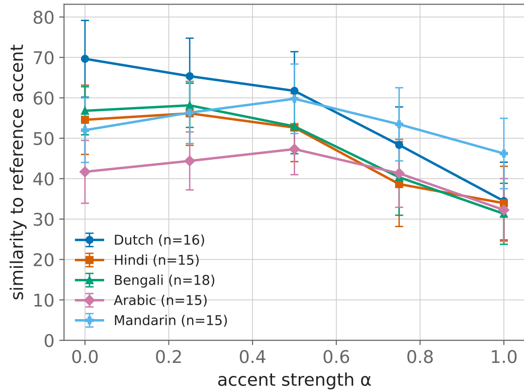
Mean rating
