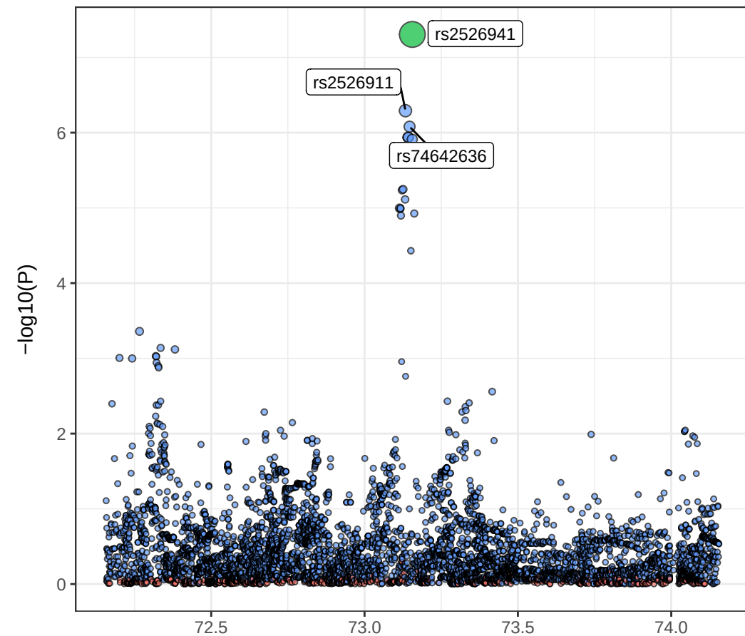
CBF_hit1_chr14 - FINEMAP
