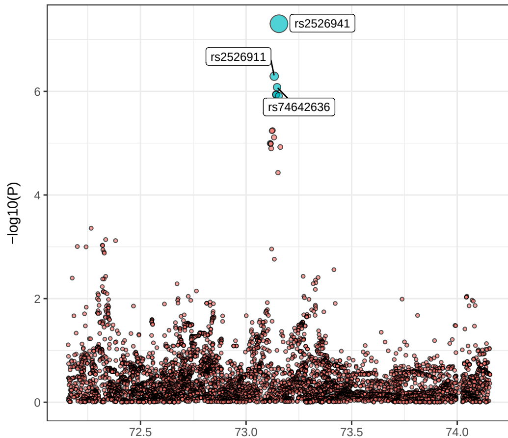
CBF_hit1_chr14 - SUSIE
