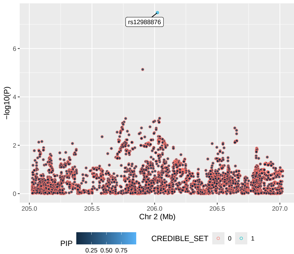
Complex_hit2_chr2 – SUSIE (sum.stats)
