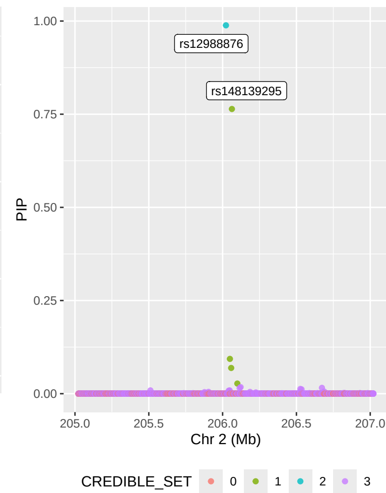
Complex_hit2_chr2 – FINEMAP (info=0.3)
