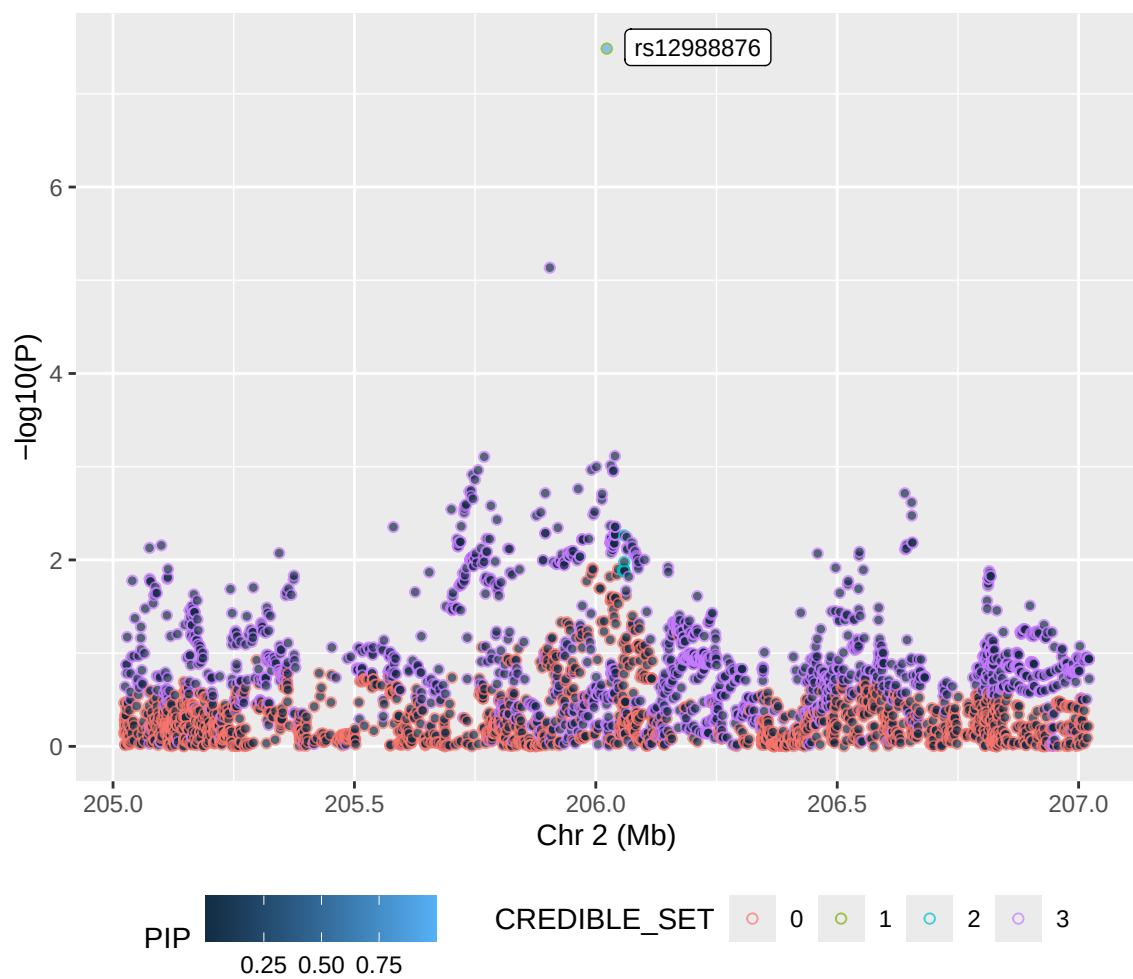
Complex_hit2_chr2 – FINEMAP (sum.stats)
