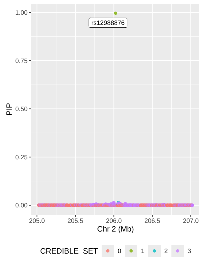
Complex_hit2_chr2 – FINEMAP (sum.stats)
