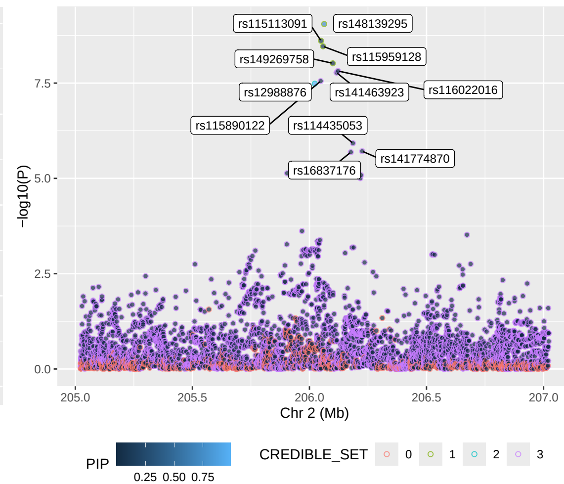
Complex_hit2_chr2 – FINEMAP (info=0.3)
