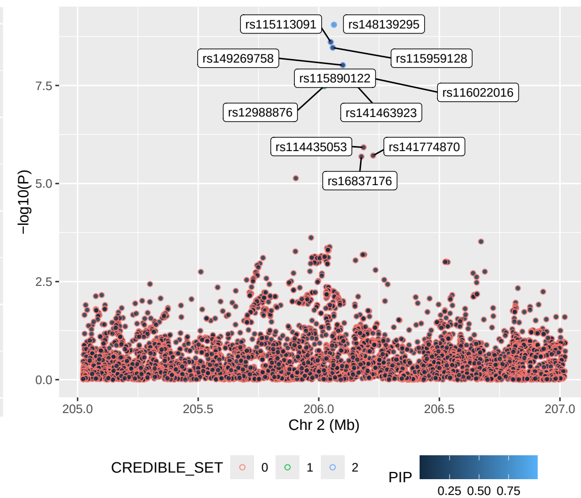
Complex_hit2_chr2 – SUSIE (info=0.3)
