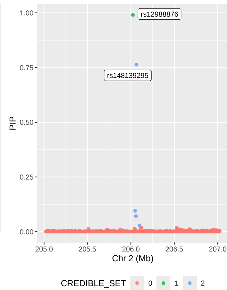
Complex_hit2_chr2 – SUSIE (info=0.3)
