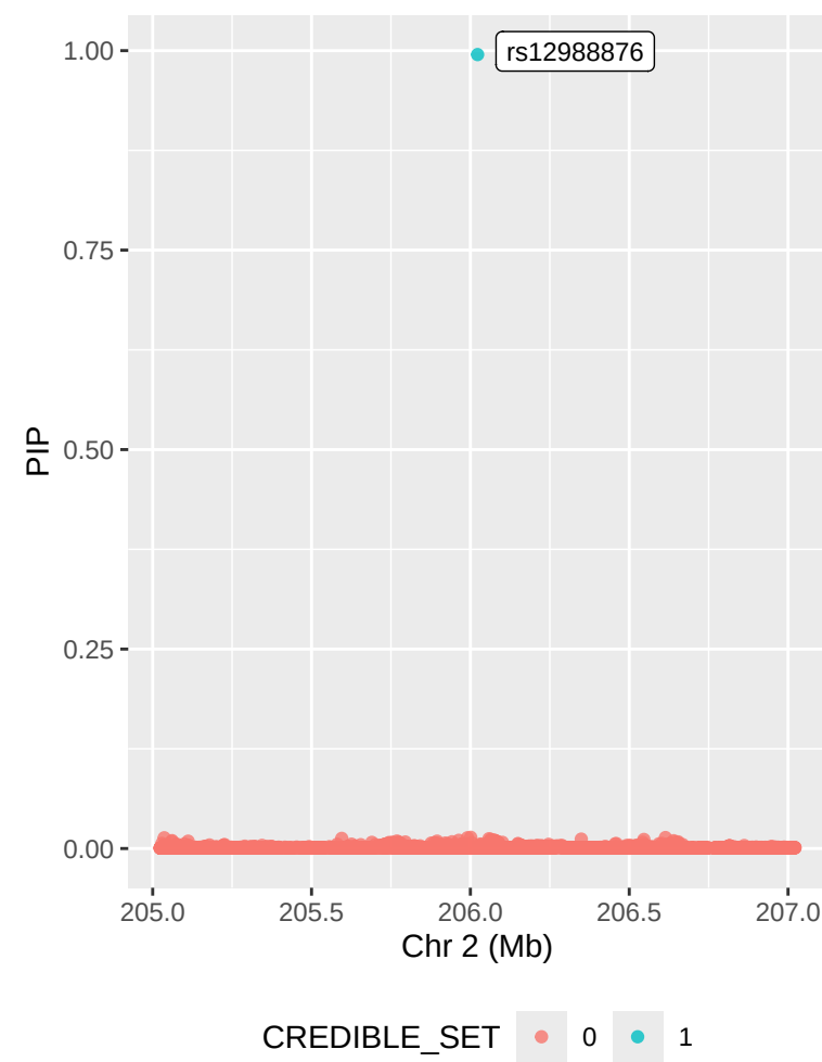
Complex_hit2_chr2 – SUSIE (sum.stats)
