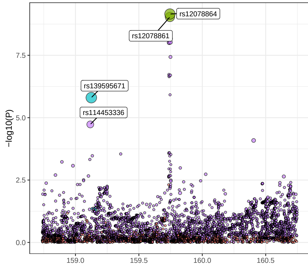
del5_7_hit1_chr1 - FINEMAP
