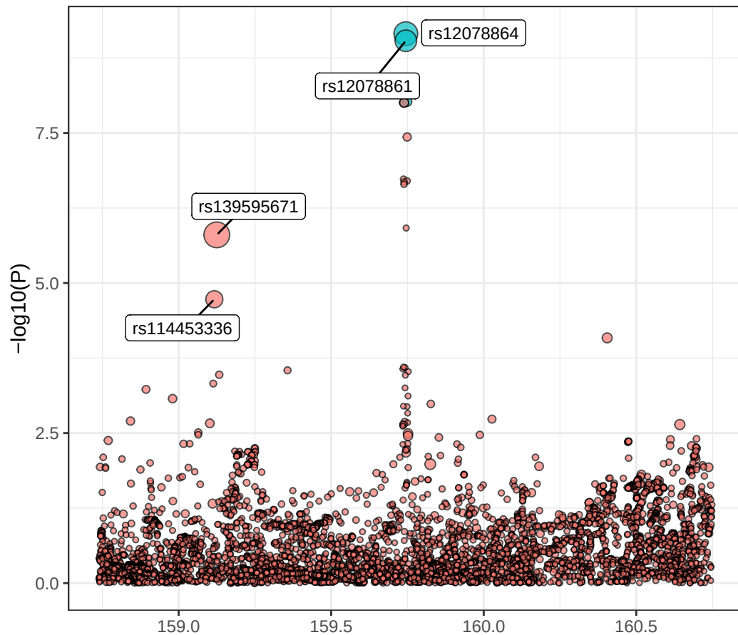
del5_7_hit1_chr1 - SUSIE
