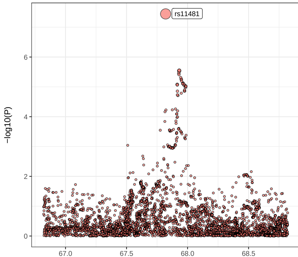
status_hit2_chr11 – SUSIE
