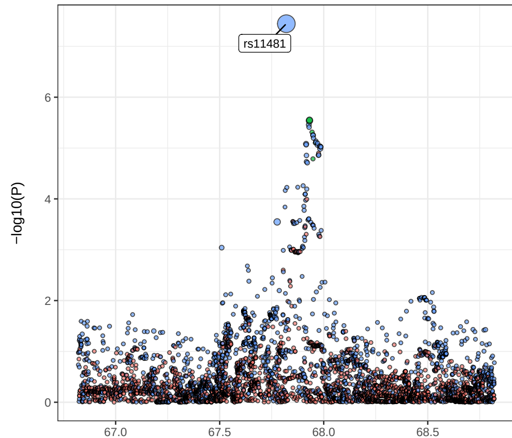
status_hit2_chr11 – FINEMAP
