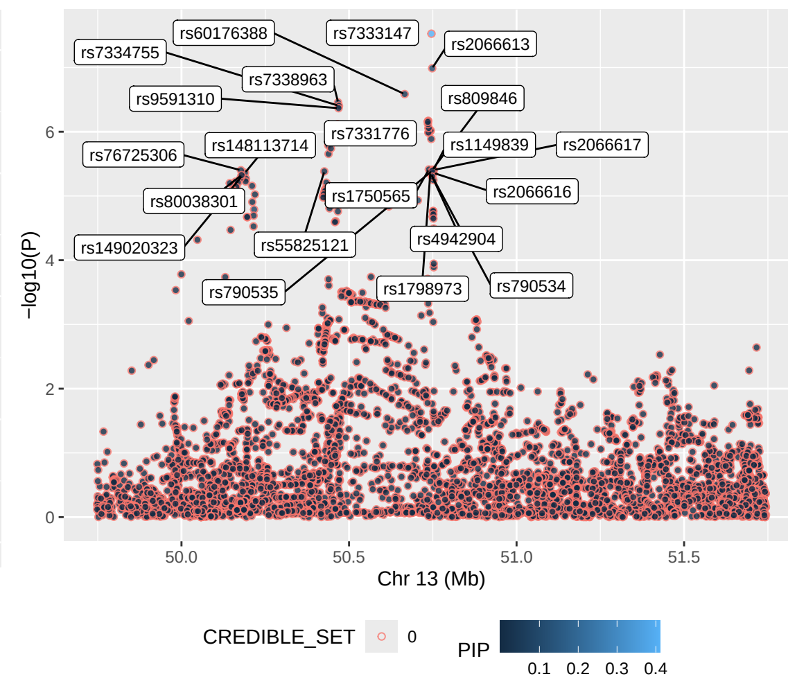
t15_17_hit1_chr13 – SUSIE (info=0.3)
