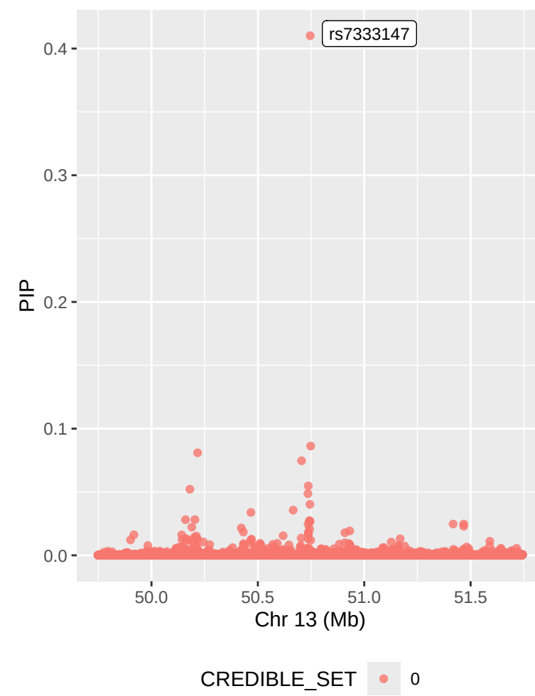
t15_17_hit1_chr13 – SUSIE (info=0.3)
