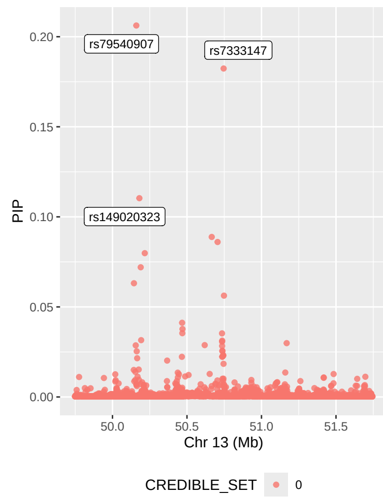
t15_17_hit1_chr13 – SUSIE (sum.stats)
