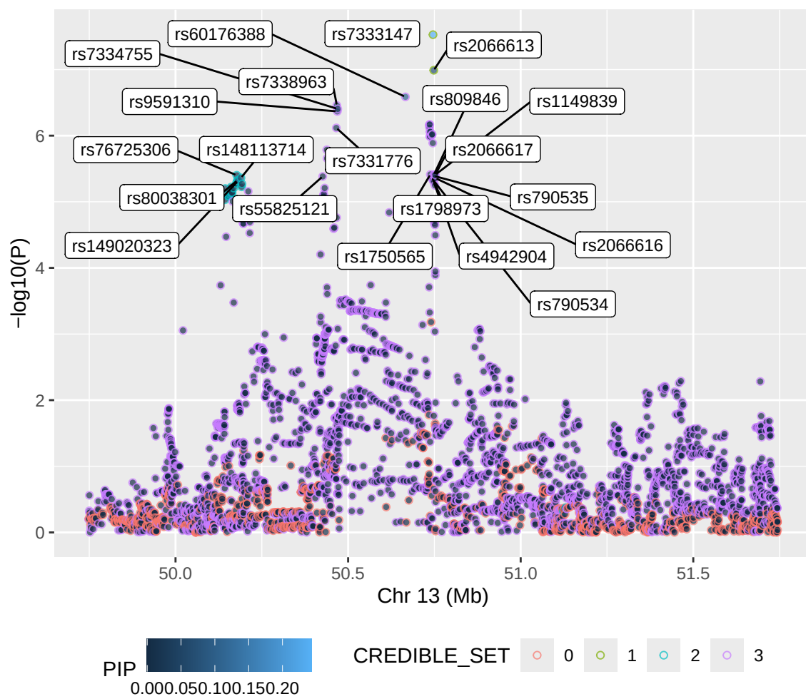
t15_17_hit1_chr13 – FINEMAP (sum.stats)
