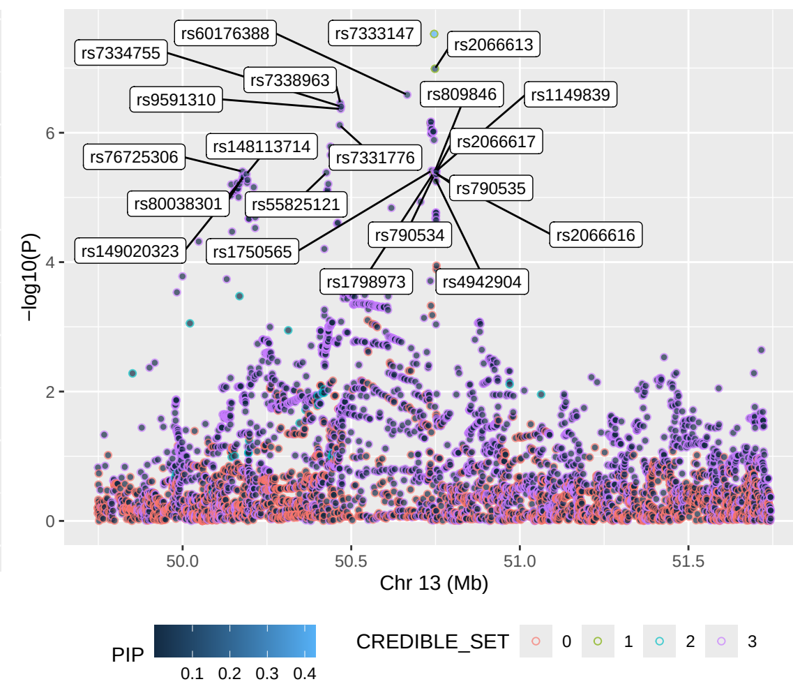
t15_17_hit1_chr13 – FINEMAP (info=0.3)
