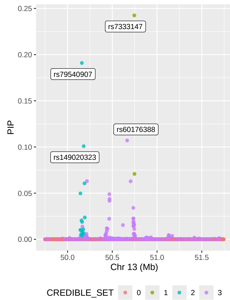
t15_17_hit1_chr13 – FINEMAP (sum.stats)
