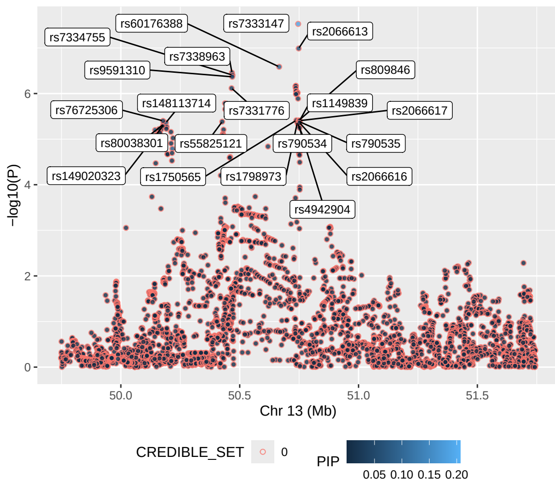
t15_17_hit1_chr13 – SUSIE (sum.stats)
