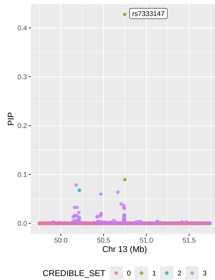
t15_17_hit1_chr13 – FINEMAP (info=0.3)
