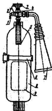
8-rasm. Karbonat angidridli o't o'chirgich
