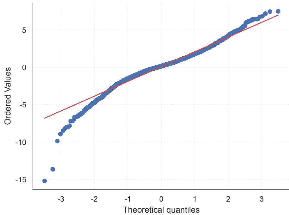
(b) KFold: normal Q-Q plot
