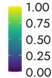
Proportion of predicted model given true model
