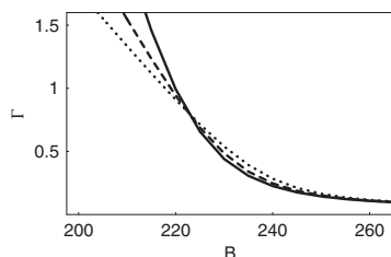
Fig. 6 Prebifurcation amplification predicted by the unfolded border-collision model (12): \delta=5 ms (solid), \delta=10 ms (dashed), and \delta=15 ms (dotted)
