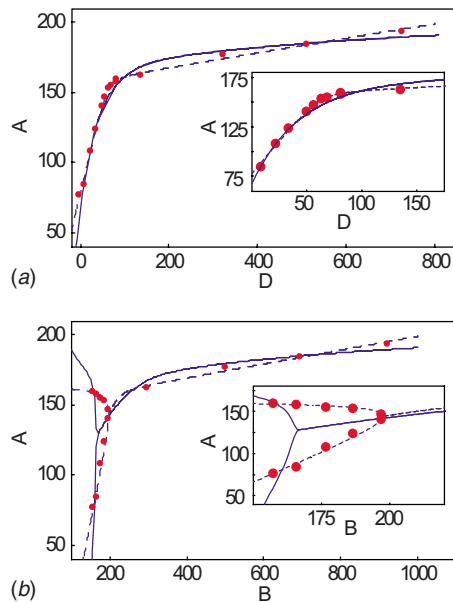
Fig. 5 Comparison between the model of Guevara et al. (solid) and the unfolded border-collision model (dashed) in fitting the experimental data in Ref. [31] (points). Although both models fit the dynamic restitution curve well (top panel), the unfolded border-collision model fits alternans data much better (bottom panel).
