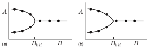
Fig. 2 Schematic bifurcation diagrams of period-doubling bifurcation: (a) a smooth type and (b) a border-collision type. Here, B represents a bifurcation parameter and A represents fixed-point solutions.
