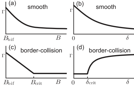
Fig. 3 Prebifurcation gain \Gamma of a classical period-doubling bifurcation ((a) and (b)) and of a border-collision period-doubling bifurcation ((c) and (d)). In Panels (a) and (c), \delta stays constant; in Panels (b) and (d), B_{\text{bif}} < B stays constant. Comparison between Panels (b) and (d) provides the most revealing difference between the two bifurcations.
