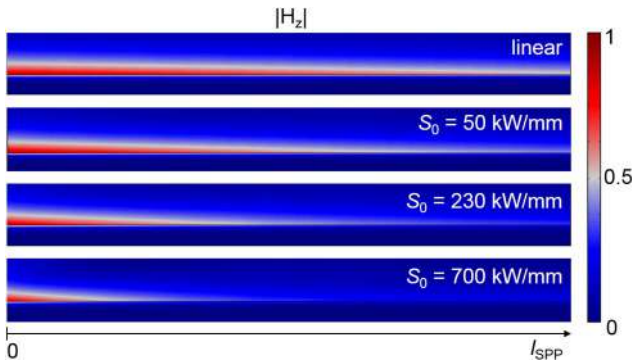
Fig. 3. Nonlinear propagation of the SPP field. Modulus of the magnetic field H_z calculated for a gold/GaAs interface at \lambda = 1.5 \mu\text{m} over a length equal to the propagation length of the surface plasmon in the linear regime for different values of S_0 . The linear and nonlinear properties of the GaAs are given in Table 1. Each plot is normalized to the input value of |H_z| .
