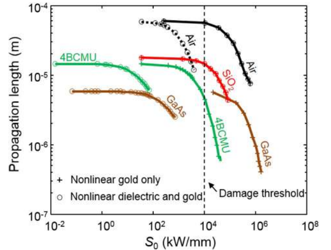
Fig. 4. Optical switching of the SPP for different gold/dielectric combinations. Propagation length of the SPP as a function of the input power per unit length S_0 for different dielectrics (black, air; red, SiO 2 ; green, 4BCMU; brown, GaAs). Crosses correspond to calculations that are carried out when only the gold nonlinear response is taken into account. Rings correspond to calculations that are carried out when the gold and dielectric nonlinear response is taken into account. The dotted curve is computed for the gold/air interface with the value of \chi^{(3)} taken from Marini et al. [19]. The dashed line indicates the optical damage threshold of gold for 100 fs pulses.
