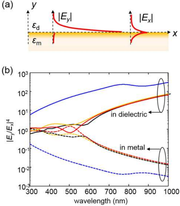
Fig. 1. Structure investigated and scaling of the electric field components. (a) Illustration of the single gold-dielectric interface. The transverse profiles of the modulus of both the y and x components of the field associated with the SPP mode are shown. (b) Spectral dependence of |E_y/E_x|^4 in the dielectric (solid lines) and in the metal (dashed lines) for \epsilon_d = 5 and for different metals (black; silver, red; gold, orange; copper and blue; aluminum).
