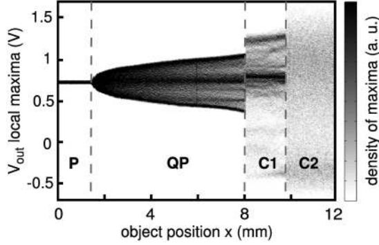
FIG. 2. Bifurcation Diagram. We store and analyze the time series of V_{\text{out}} at each object position along a 1D path in the x direction. The local maxima of each time series is plotted as a function of object position x .
