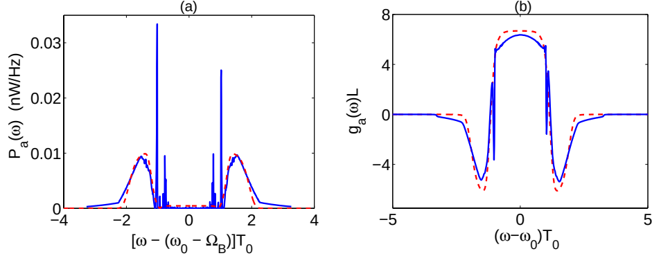
Fig. 6. (a) Optimal absorption pump profile (solid) and super-Gaussian fit (dash) and (b) gain+absorption profile (solid) and super-Gaussian fit (dash) for gain+absorption medium using super-Gaussian pulse spectrum and T_{\text{pulse}}=250 ps.
