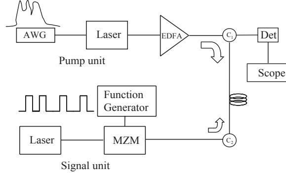
Fig. 1. Arbitray pump broadened slow-light system.
