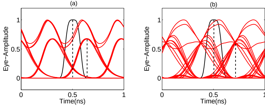
Fig. 9. Output eye diagrams for (a) GNPB medium and (b) optimal gain-only medium using a super-Gaussian RZ pulse sequence and 1/e FWHM pulse width T_{\text{pulse}} = 166 ps.
