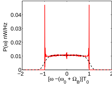
Fig. 4. Optimal pump profile (solid) and super-Gaussian fit (dash) for gain-only medium using super-Gaussian pulse spectrum and T_{\text{pulse}}=166 ps.
