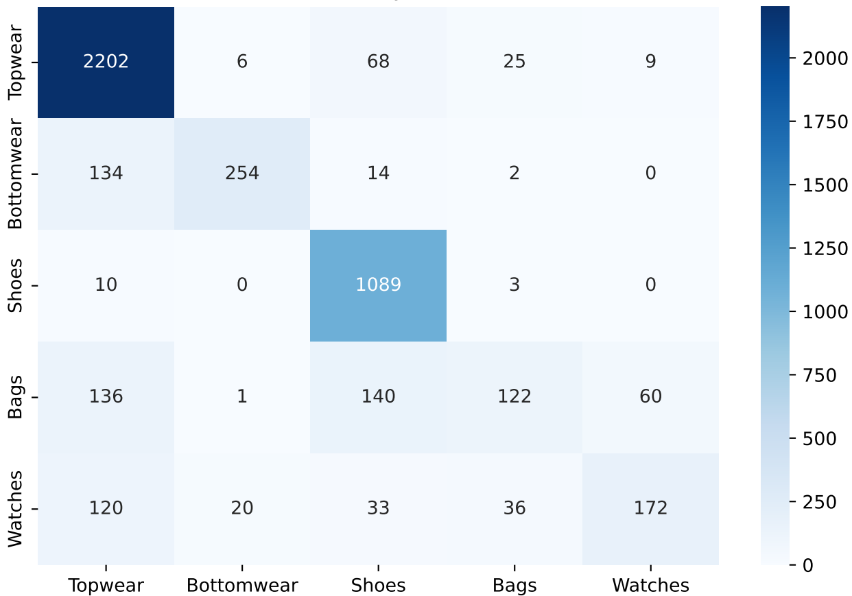
Custom Architecture Analytical Confusion Matrix
