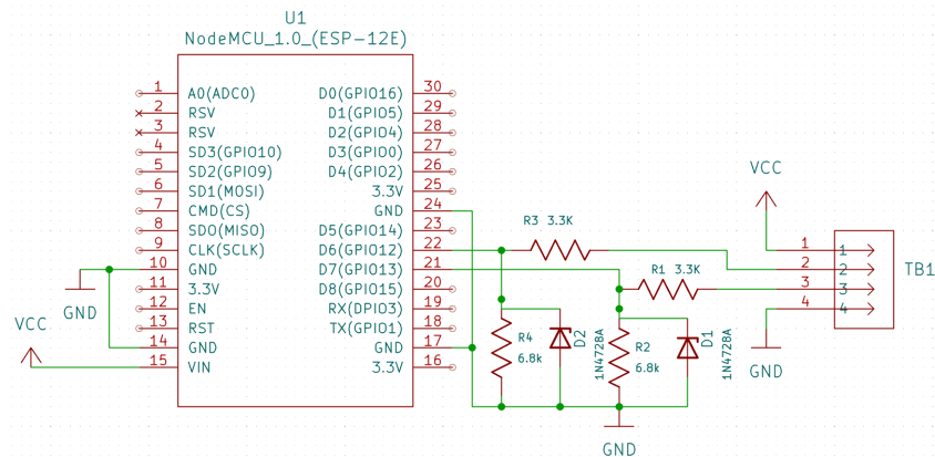
Figure 6.2: RFID Controller
