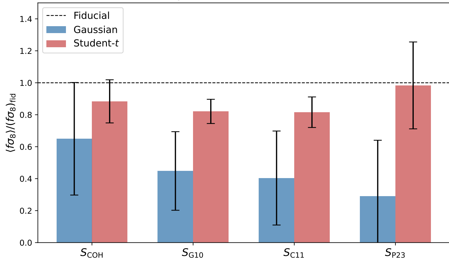
f\sigma_8 recovery: Gaussian vs Student- t likelihood
